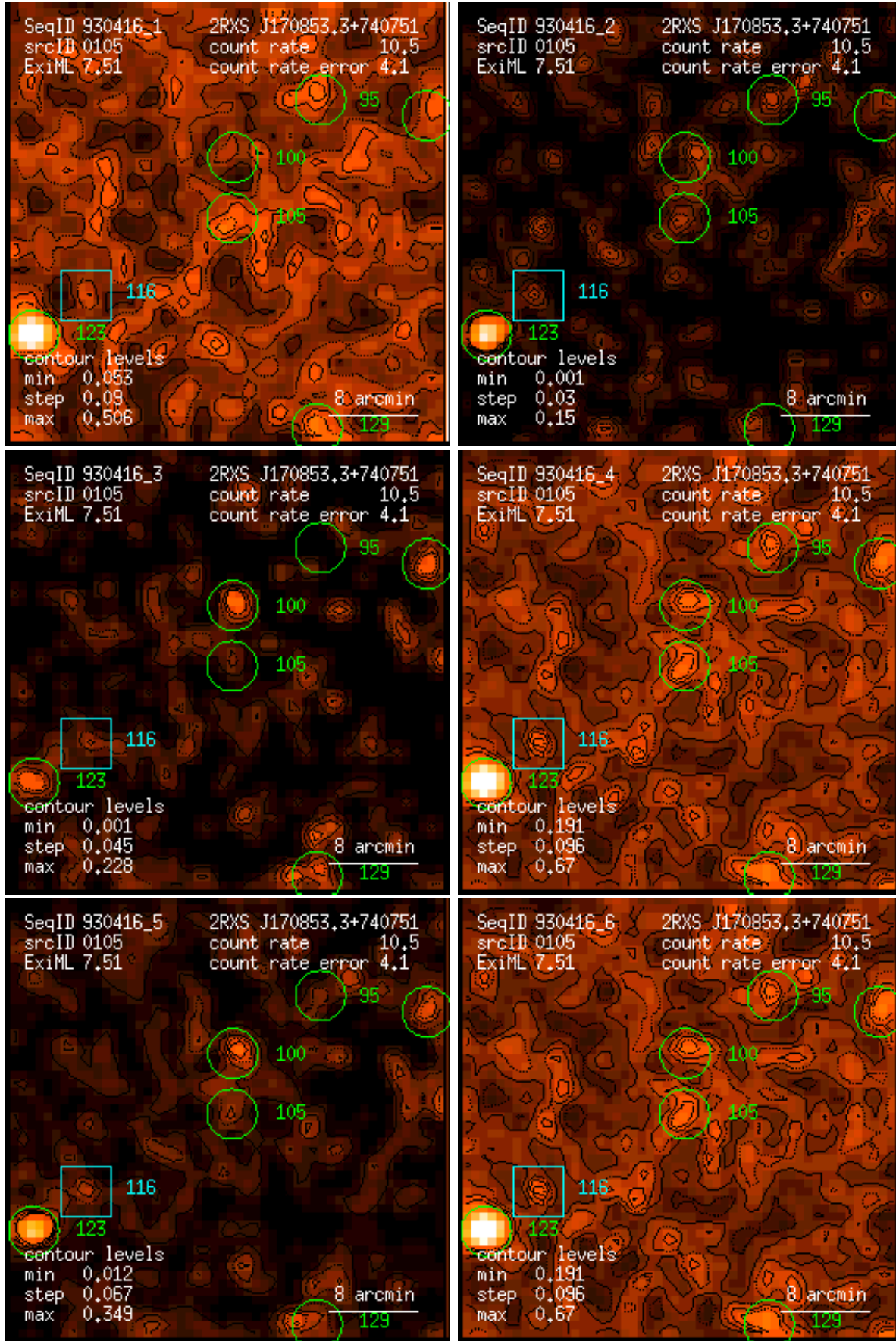
Figure 105: RASS 930416: detection 0105: band rate images, Gaussian filter: (1) PSPC channels 11 – 41, (2) 52 – 90, (3) 91 – 201, (4) 11 – 235, (5) 52 – 201, (6) 11 – 201. Broad band rates in counts/ks. Band rate contour levels in counts/ks/arcmin 2 .
