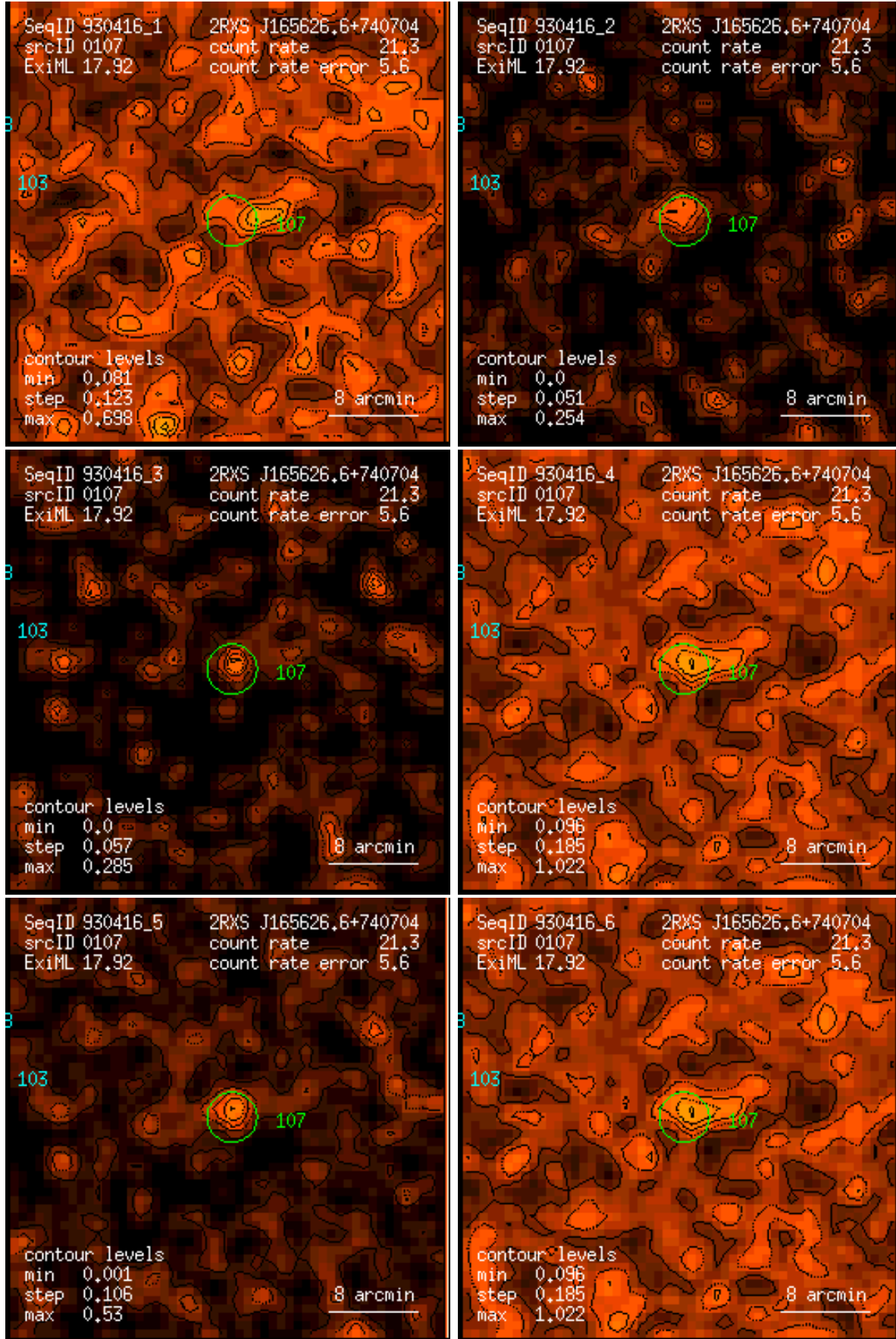
Figure 107: RASS 930416: detection 0107: band rate images, Gaussian filter: (1) PSPC channels 11 – 41, (2) 52 – 90, (3) 91 – 201, (4) 11 – 235, (5) 52 – 201, (6) 11 – 201. Broad band rates in counts/ks. Band rate contour levels in counts/ks/arcmin 2 .
