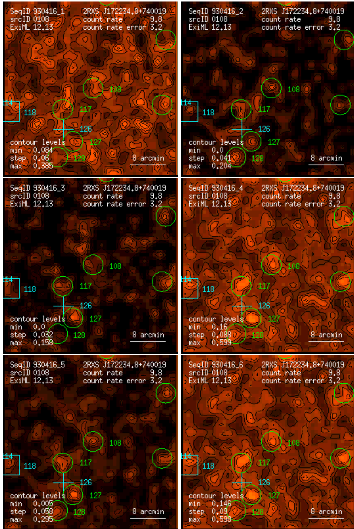
Figure 108: RASS 930416: detection 0108: band rate images, Gaussian filter: (1) PSPC channels 11 – 41, (2) 52 – 90, (3) 91 – 201, (4) 11 – 235, (5) 52 – 201, (6) 11 – 201. Broad band rates in counts/ks. Band rate contour levels in counts/ks/arcmin 2 .
