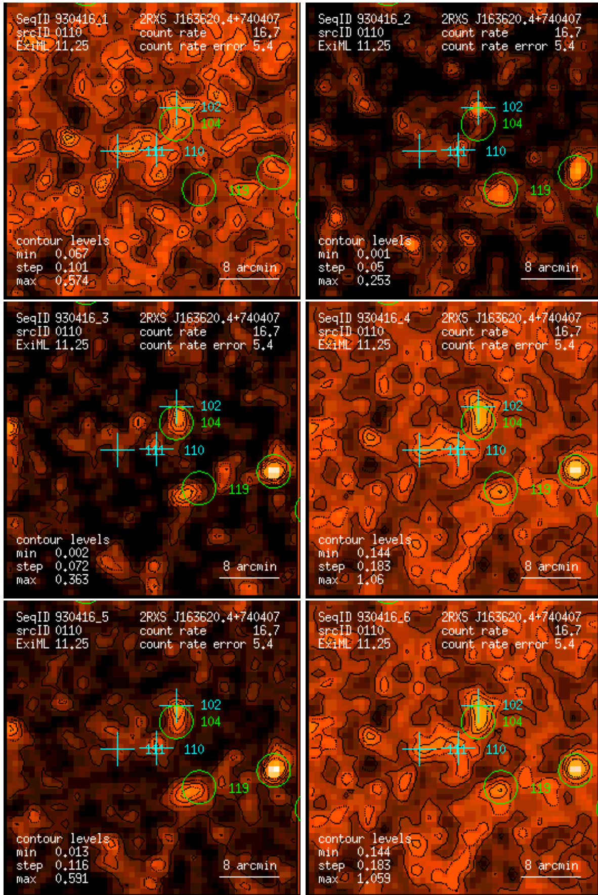
Figure 110: RASS 930416: detection 0110: band rate images, Gaussian filter: (1) PSPC channels 11 – 41, (2) 52 – 90, (3) 91 – 201, (4) 11 – 235, (5) 52 – 201, (6) 11 – 201. Broad band rates in counts/ks. Band rate contour levels in counts/ks/arcmin 2 .
