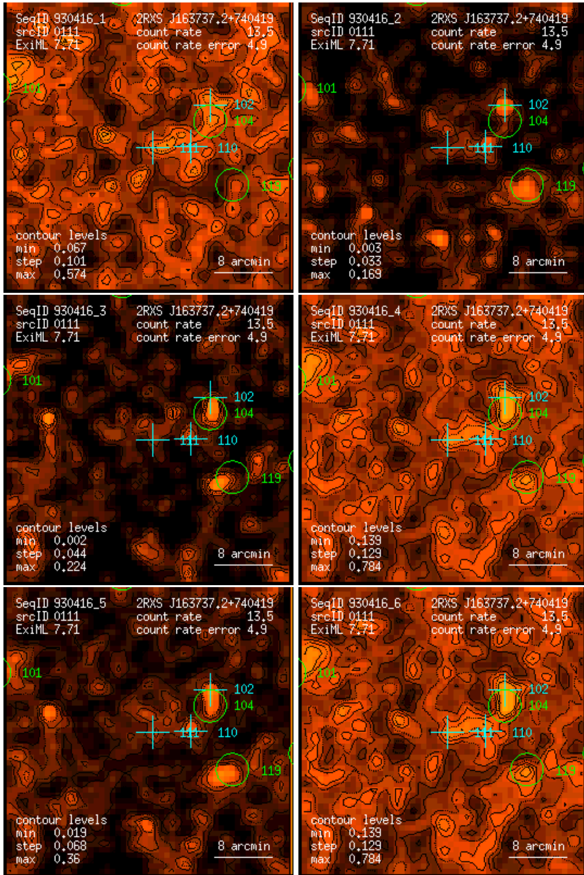
Figure 111: RASS 930416: detection 0111: band rate images, Gaussian filter: (1) PSPC channels 11 – 41, (2) 52 – 90, (3) 91 – 201, (4) 11 – 235, (5) 52 – 201, (6) 11 – 201. Broad band rates in counts/ks. Band rate contour levels in counts/ks/arcmin 2 .
