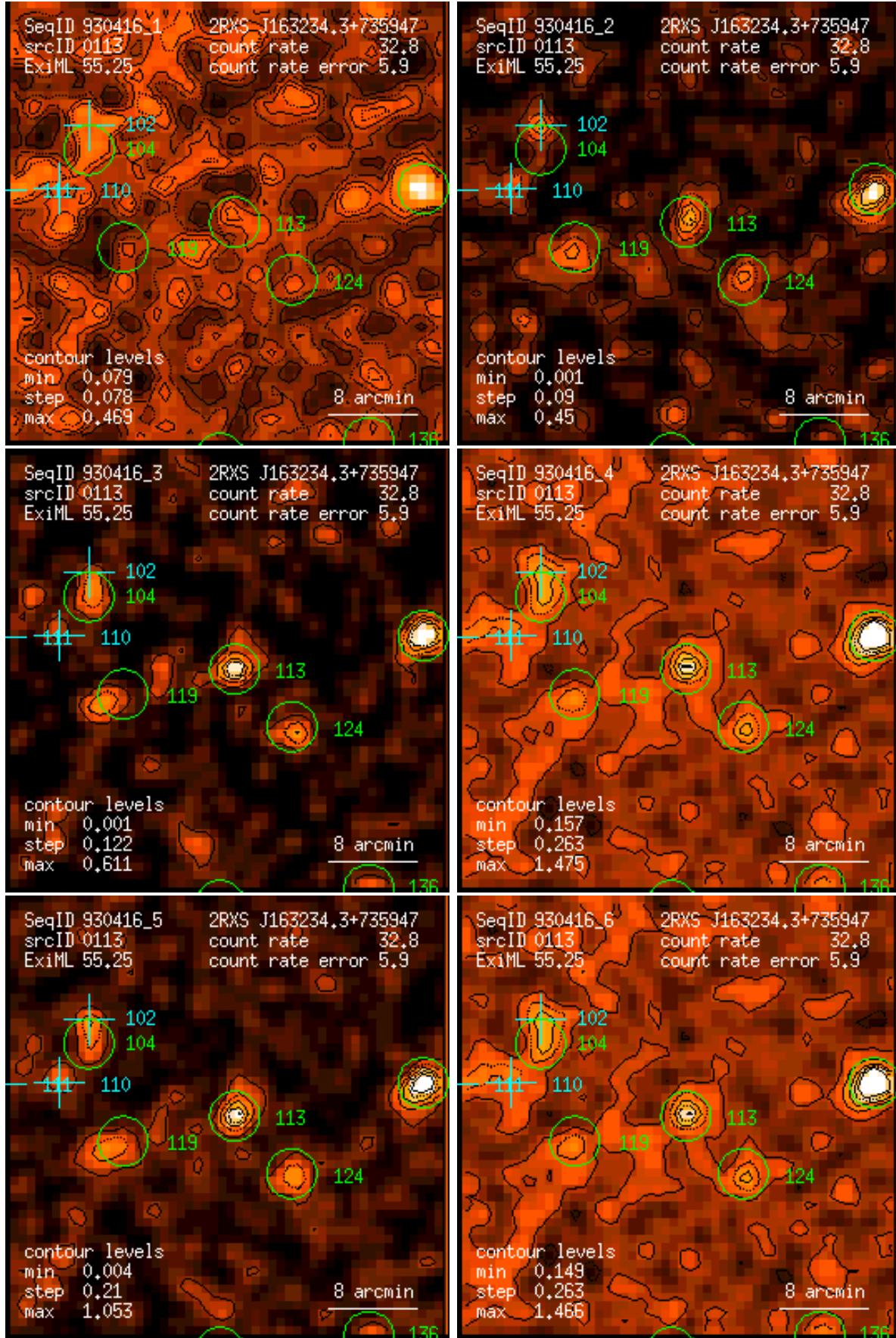
Figure 113: RASS 930416: detection 0113: band rate images, Gaussian filter: (1) PSPC channels 11 – 41, (2) 52 – 90, (3) 91 – 201, (4) 11 – 235, (5) 52 – 201, (6) 11 – 201. Broad band rates in counts/ks. Band rate contour levels in counts/ks/arcmin 2 .
