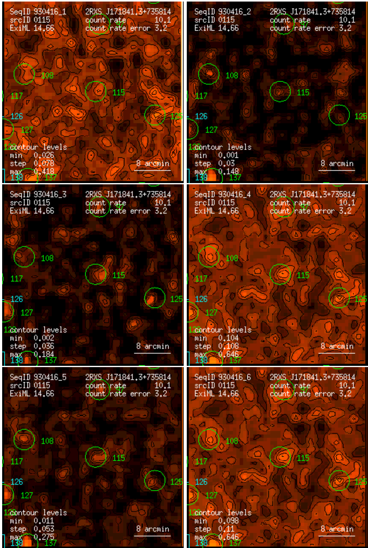
Figure 115: RASS 930416: detection 0115: band rate images, Gaussian filter: (1) PSPC channels 11 – 41, (2) 52 – 90, (3) 91 – 201, (4) 11 – 235, (5) 52 – 201, (6) 11 – 201. Broad band rates in counts/ks. Band rate contour levels in counts/ks/arcmin 2 .
