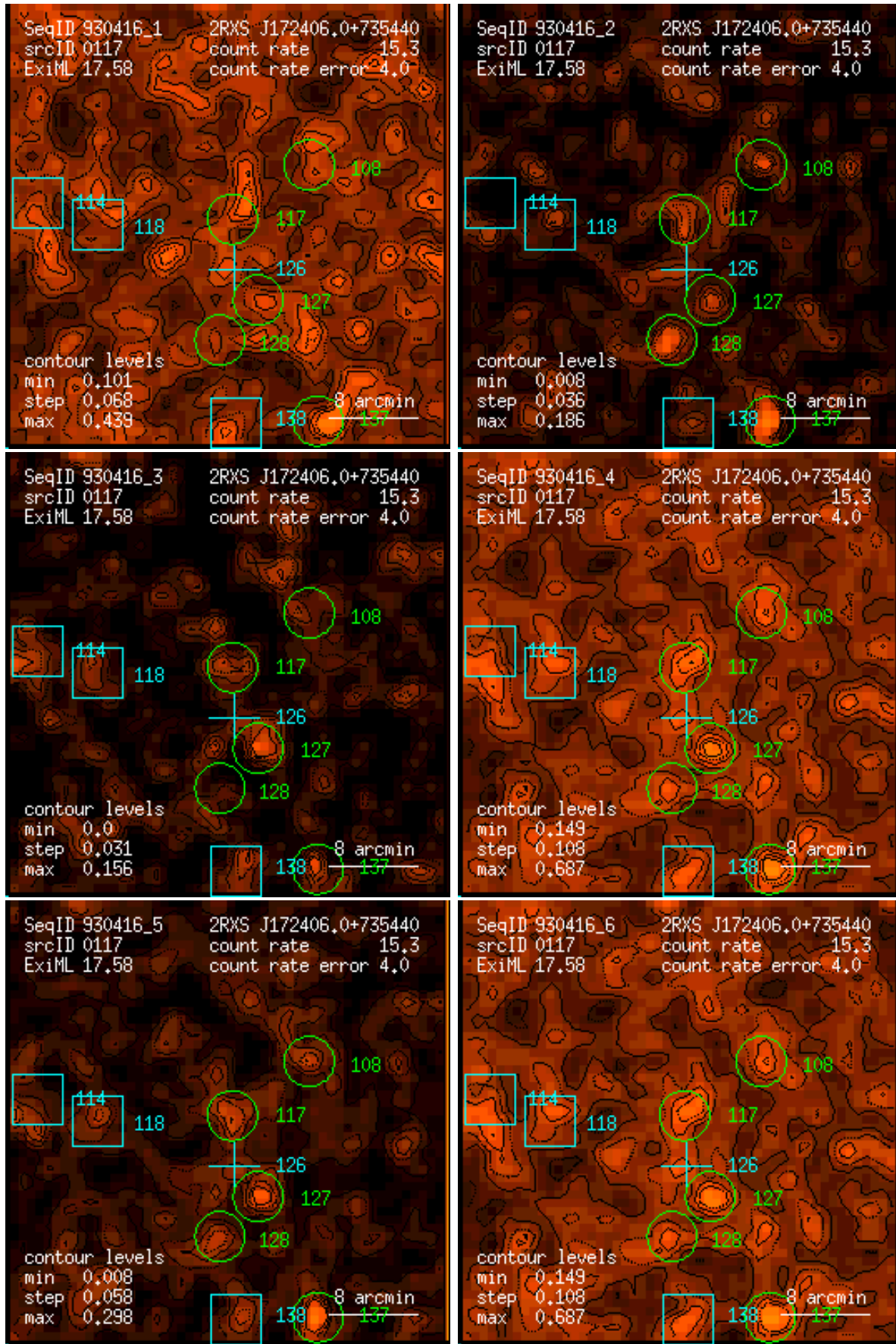
Figure 117: RASS 930416: detection 0117: band rate images, Gaussian filter: (1) PSPC channels 11 – 41, (2) 52 – 90, (3) 91 – 201, (4) 11 – 235, (5) 52 – 201, (6) 11 – 201. Broad band rates in counts/ks. Band rate contour levels in counts/ks/arcmin 2 .
