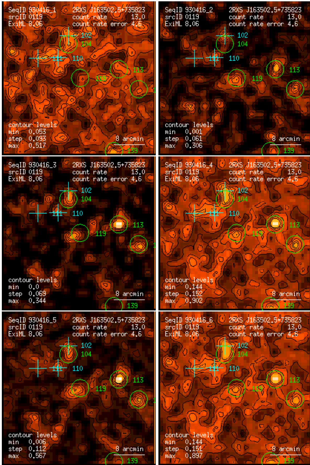
Figure 119: RASS 930416: detection 0119: band rate images, Gaussian filter: (1) PSPC channels 11 – 41, (2) 52 – 90, (3) 91 – 201, (4) 11 – 235, (5) 52 – 201, (6) 11 – 201. Broad band rates in counts/ks. Band rate contour levels in counts/ks/arcmin 2 .
