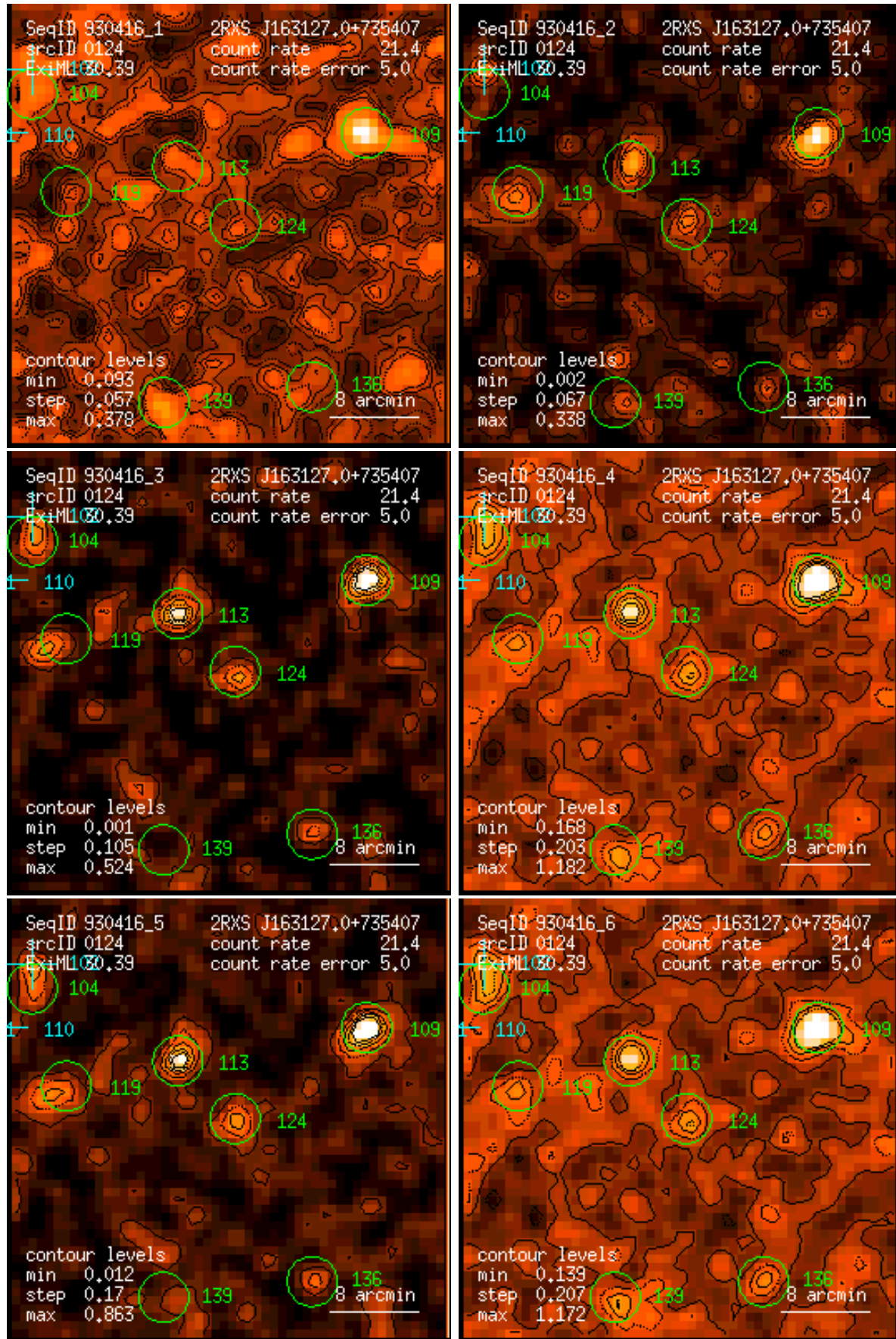
Figure 124: RASS 930416: detection 0124: band rate images, Gaussian filter: (1) PSPC channels 11 – 41, (2) 52 – 90, (3) 91 – 201, (4) 11 – 235, (5) 52 – 201, (6) 11 – 201. Broad band rates in counts/ks. Band rate contour levels in counts/ks/arcmin 2 .
