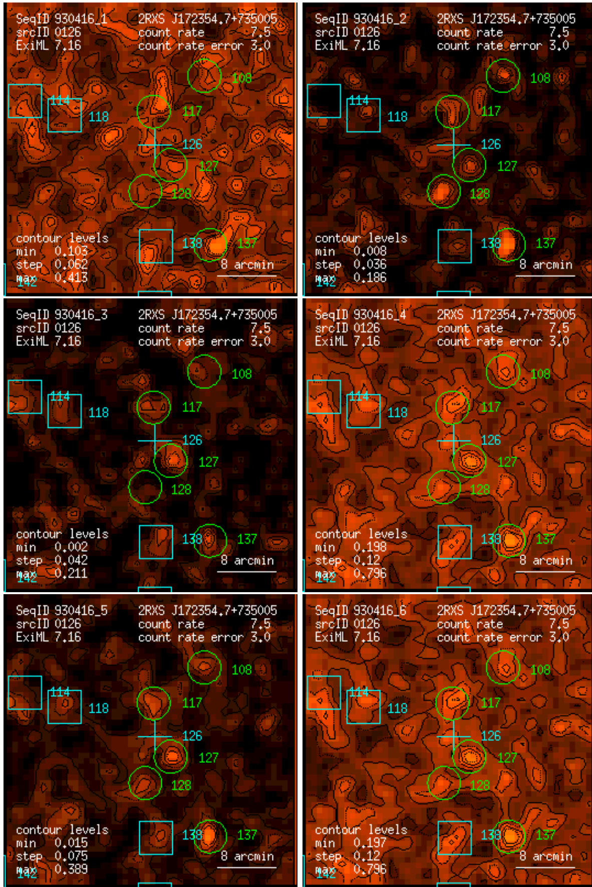
Figure 126: RASS 930416: detection 0126: band rate images, Gaussian filter: (1) PSPC channels 11 – 41, (2) 52 – 90, (3) 91 – 201, (4) 11 – 235, (5) 52 – 201, (6) 11 – 201. Broad band rates in counts/ks. Band rate contour levels in counts/ks/arcmin 2 .
