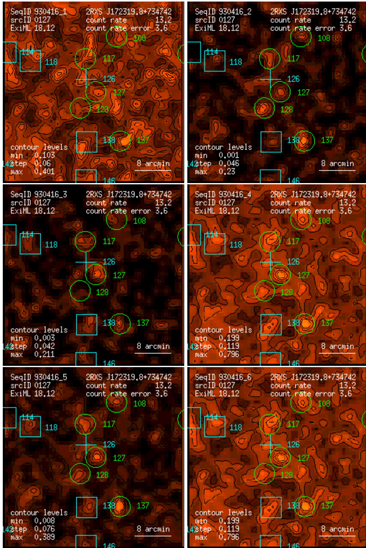
Figure 127: RASS 930416: detection 0127: band rate images, Gaussian filter: (1) PSPC channels 11 – 41, (2) 52 – 90, (3) 91 – 201, (4) 11 – 235, (5) 52 – 201, (6) 11 – 201. Broad band rates in counts/ks. Band rate contour levels in counts/ks/arcmin 2 .
