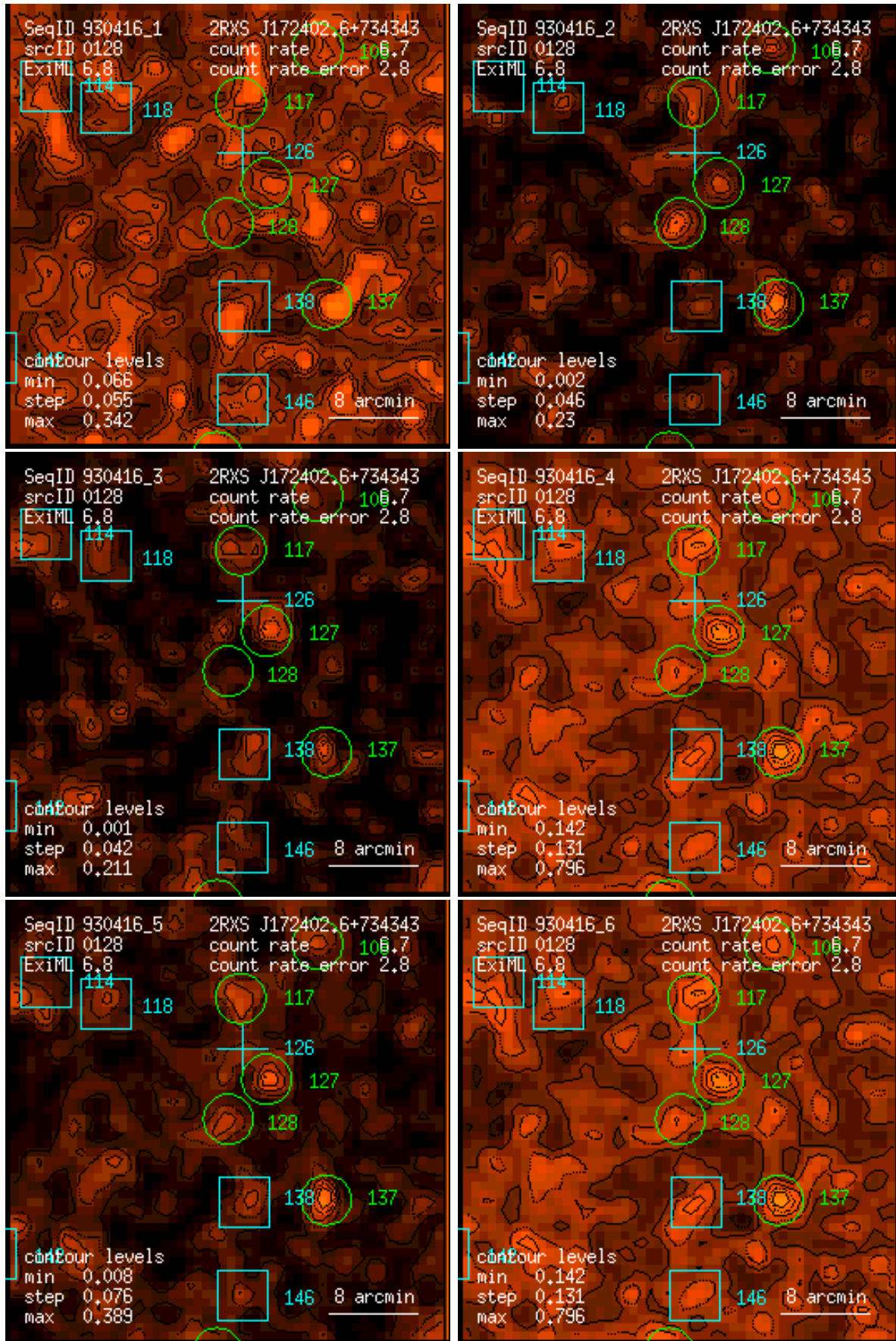
Figure 128: RASS 930416: detection 0128: band rate images, Gaussian filter: (1) PSPC channels 11 – 41, (2) 52 – 90, (3) 91 – 201, (4) 11 – 235, (5) 52 – 201, (6) 11 – 201. Broad band rates in counts/ks. Band rate contour levels in counts/ks/arcmin 2 .
