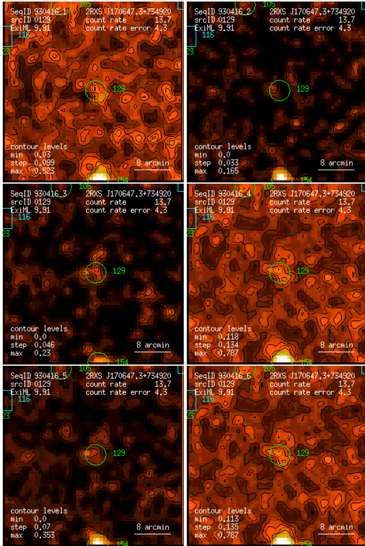
Figure 129: RASS 930416: detection 0129: band rate images, Gaussian filter: (1) PSPC channels 11 – 41, (2) 52 – 90, (3) 91 – 201, (4) 11 – 235, (5) 52 – 201, (6) 11 – 201. Broad band rates in counts/ks. Band rate contour levels in counts/ks/arcmin 2 .
