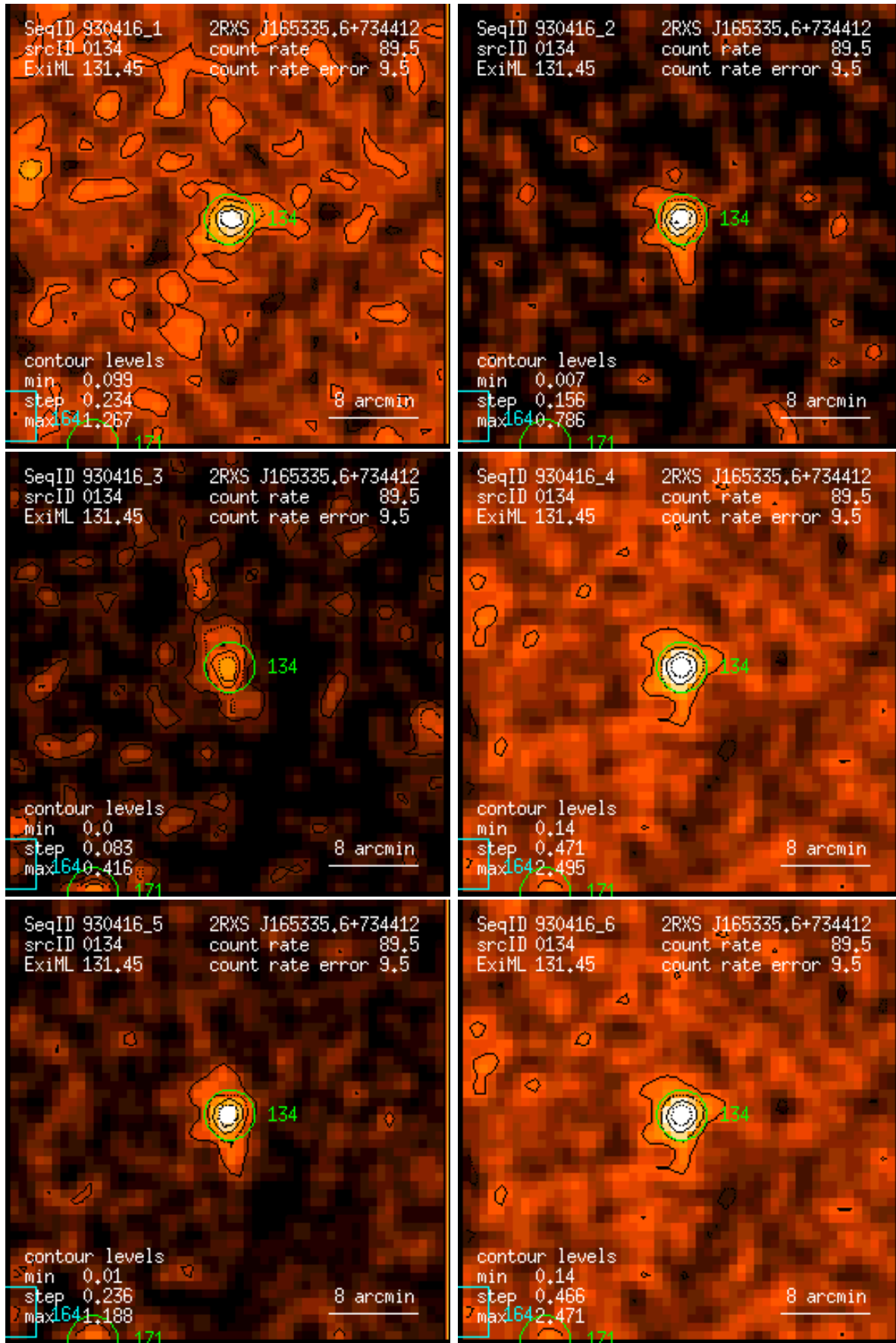
Figure 134: RASS 930416: detection 0134: band rate images, Gaussian filter: (1) PSPC channels 11 – 41, (2) 52 – 90, (3) 91 – 201, (4) 11 – 235, (5) 52 – 201, (6) 11 – 201. Broad band rates in counts/ks. Band rate contour levels in counts/ks/arcmin 2 .
