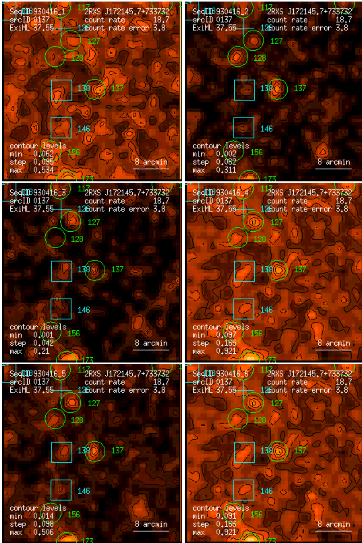
Figure 137: RASS 930416: detection 0137: band rate images, Gaussian filter: (1) PSPC channels 11 – 41, (2) 52 – 90, (3) 91 – 201, (4) 11 – 235, (5) 52 – 201, (6) 11 – 201. Broad band rates in counts/ks. Band rate contour levels in counts/ks/arcmin 2 .
