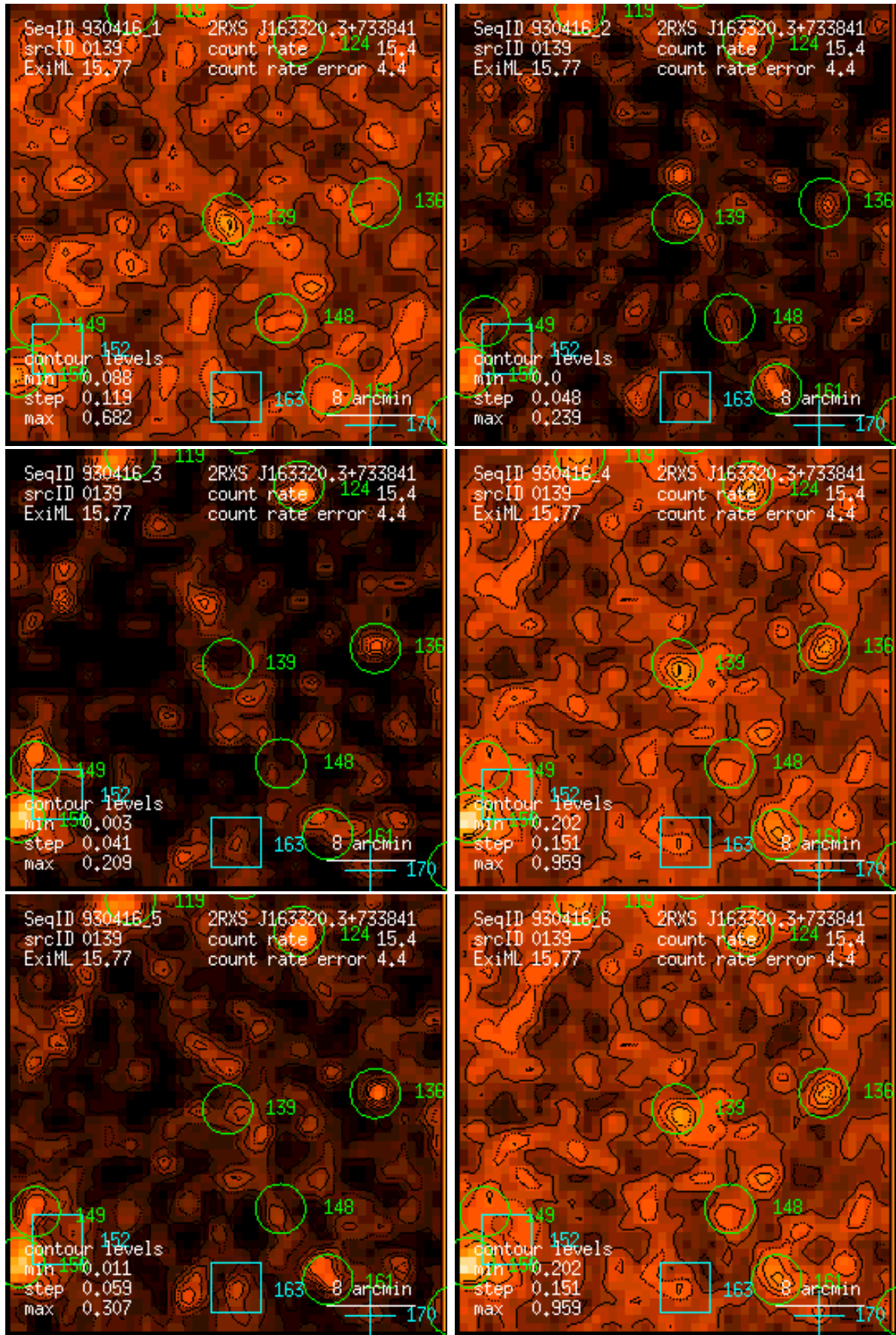
Figure 139: RASS 930416: detection 0139: band rate images, Gaussian filter: (1) PSPC channels 11 – 41, (2) 52 – 90, (3) 91 – 201, (4) 11 – 235, (5) 52 – 201, (6) 11 – 201. Broad band rates in counts/ks. Band rate contour levels in counts/ks/arcmin 2 .
