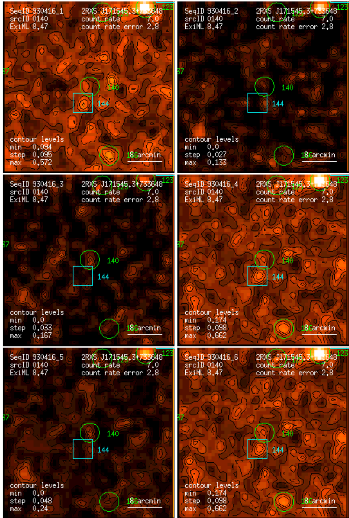
Figure 140: RASS 930416: detection 0140: band rate images, Gaussian filter: (1) PSPC channels 11 – 41, (2) 52 – 90, (3) 91 – 201, (4) 11 – 235, (5) 52 – 201, (6) 11 – 201. Broad band rates in counts/ks. Band rate contour levels in counts/ks/arcmin 2 .
