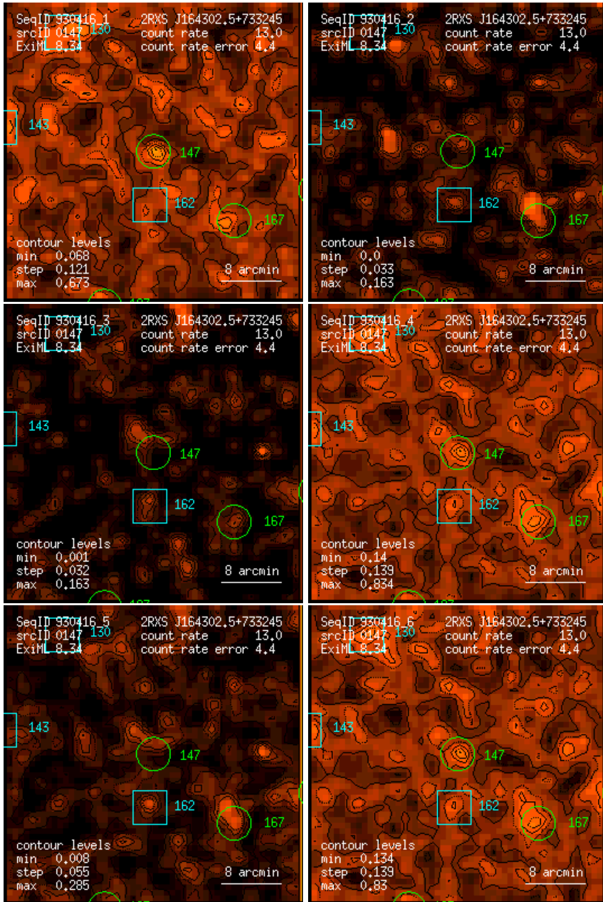
Figure 147: RASS 930416: detection 0147: band rate images, Gaussian filter: (1) PSPC channels 11 – 41, (2) 52 – 90, (3) 91 – 201, (4) 11 – 235, (5) 52 – 201, (6) 11 – 201. Broad band rates in counts/ks. Band rate contour levels in counts/ks/arcmin 2 .
