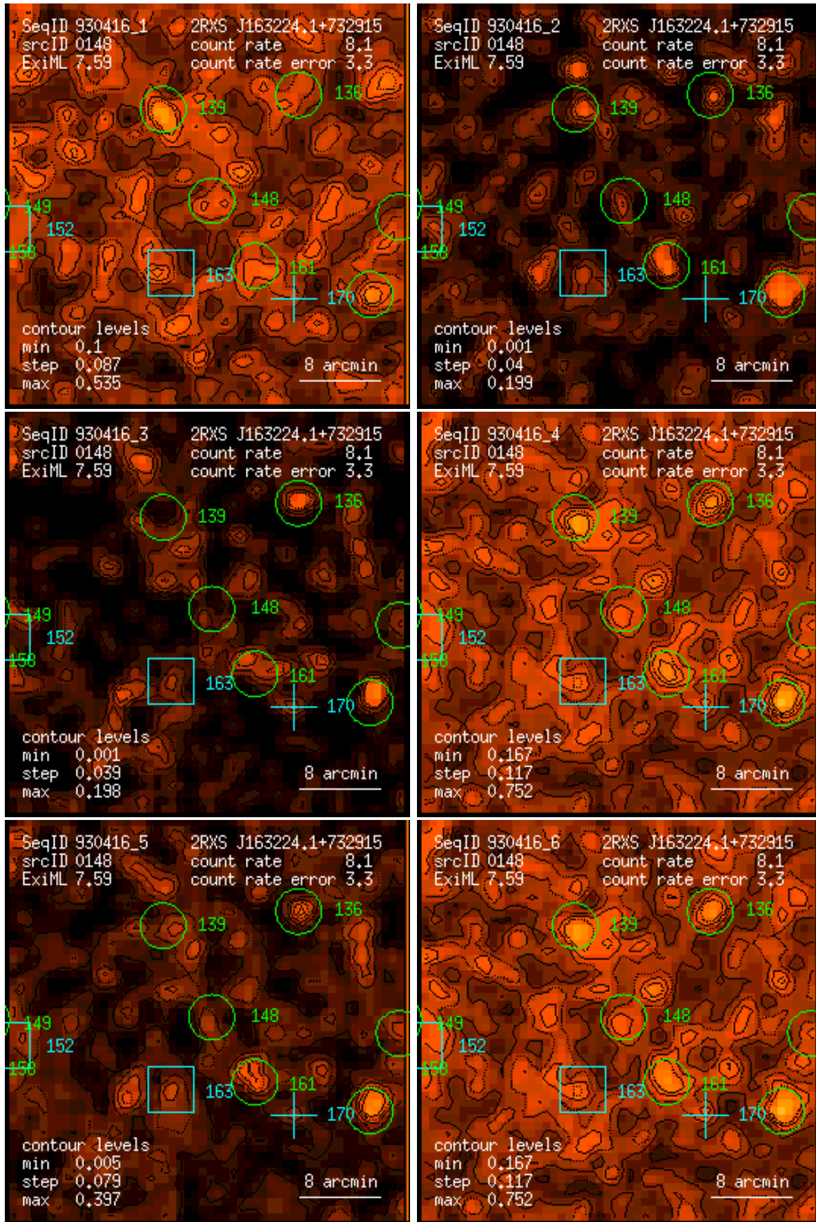
Figure 148: RASS 930416: detection 0148: band rate images, Gaussian filter: (1) PSPC channels 11 – 41, (2) 52 – 90, (3) 91 – 201, (4) 11 – 235, (5) 52 – 201, (6) 11 – 201. Broad band rates in counts/ks. Band rate contour levels in counts/ks/arcmin 2 .
