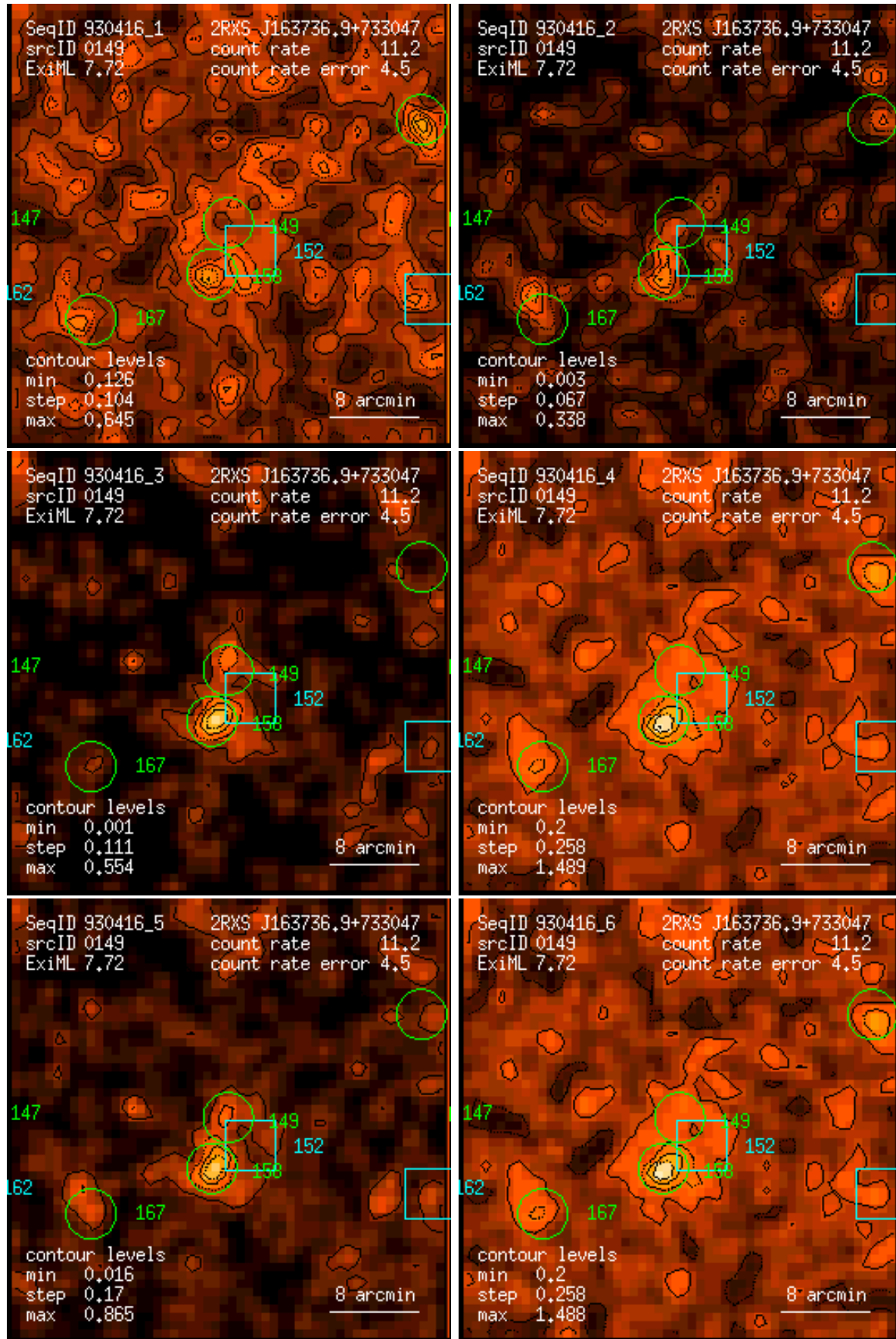
Figure 149: RASS 930416: detection 0149: band rate images, Gaussian filter: (1) PSPC channels 11 – 41, (2) 52 – 90, (3) 91 – 201, (4) 11 – 235, (5) 52 – 201, (6) 11 – 201. Broad band rates in counts/ks. Band rate contour levels in counts/ks/arcmin 2 .
