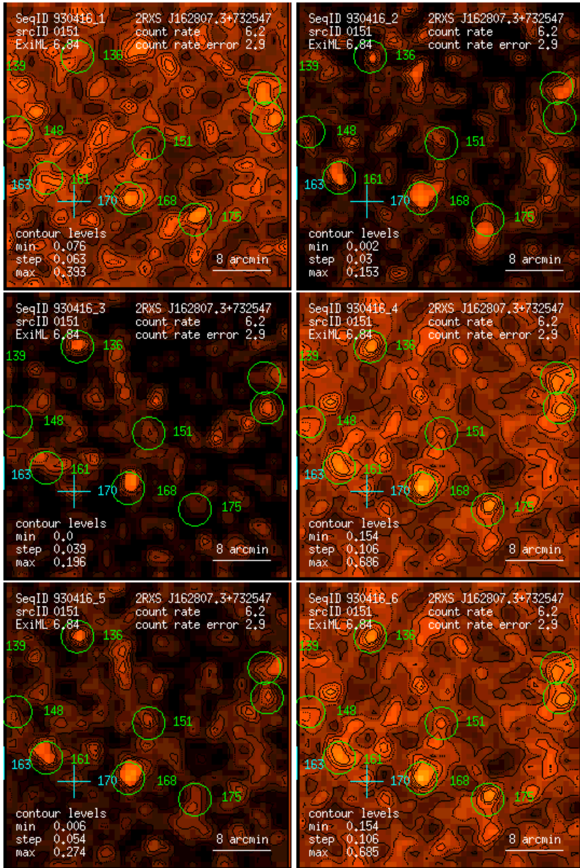
Figure 151: RASS 930416: detection 0151: band rate images, Gaussian filter: (1) PSPC channels 11 – 41, (2) 52 – 90, (3) 91 – 201, (4) 11 – 235, (5) 52 – 201, (6) 11 – 201. Broad band rates in counts/ks. Band rate contour levels in counts/ks/arcmin 2 .
