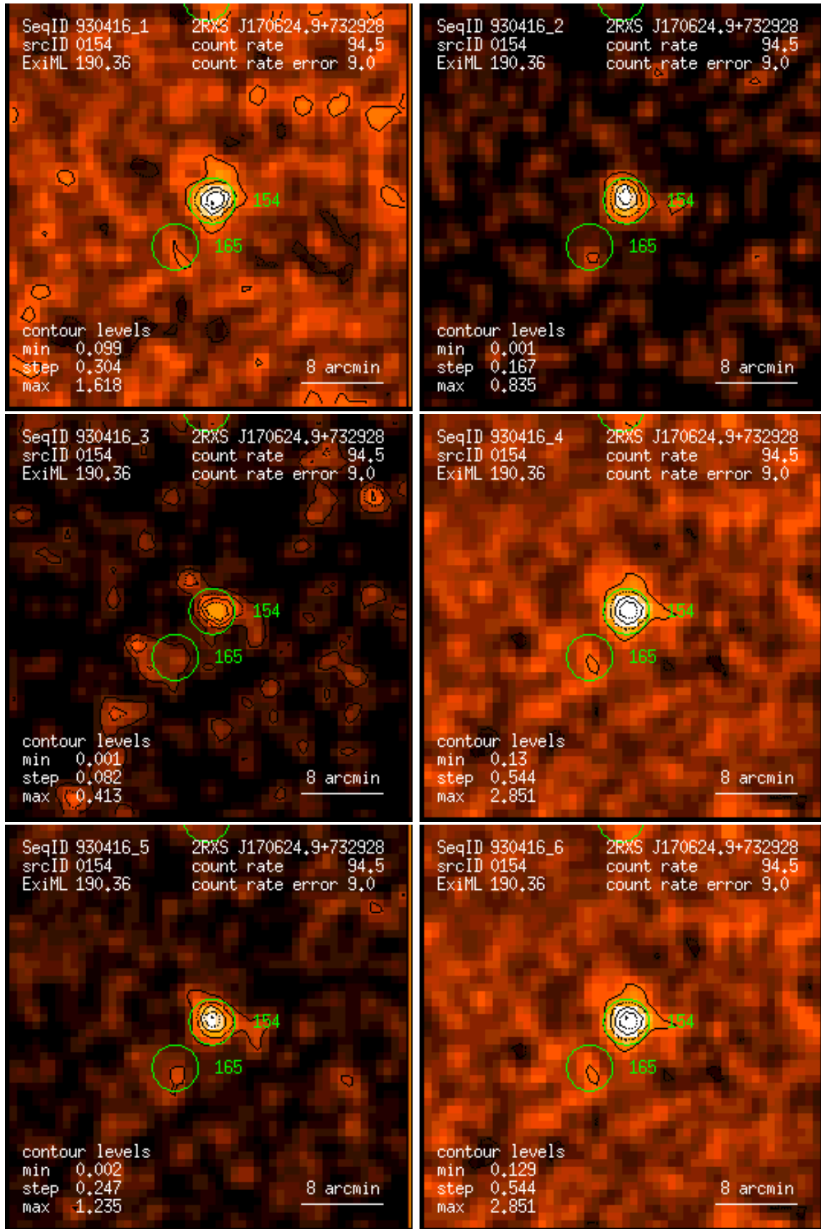
Figure 154: RASS 930416: detection 0154: band rate images, Gaussian filter: (1) PSPC channels 11 – 41, (2) 52 – 90, (3) 91 – 201, (4) 11 – 235, (5) 52 – 201, (6) 11 – 201. Broad band rates in counts/ks. Band rate contour levels in counts/ks/arcmin 2 .
