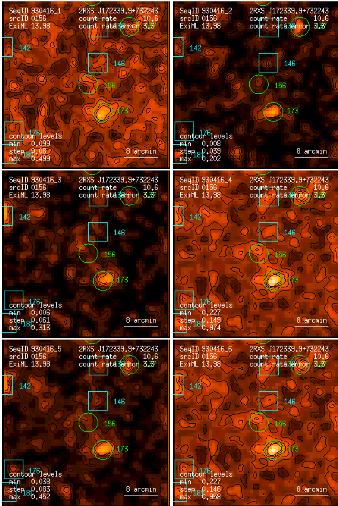
Figure 156: RASS 930416: detection 0156: band rate images, Gaussian filter: (1) PSPC channels 11 – 41, (2) 52 – 90, (3) 91 – 201, (4) 11 – 235, (5) 52 – 201, (6) 11 – 201. Broad band rates in counts/ks. Band rate contour levels in counts/ks/arcmin 2 .
