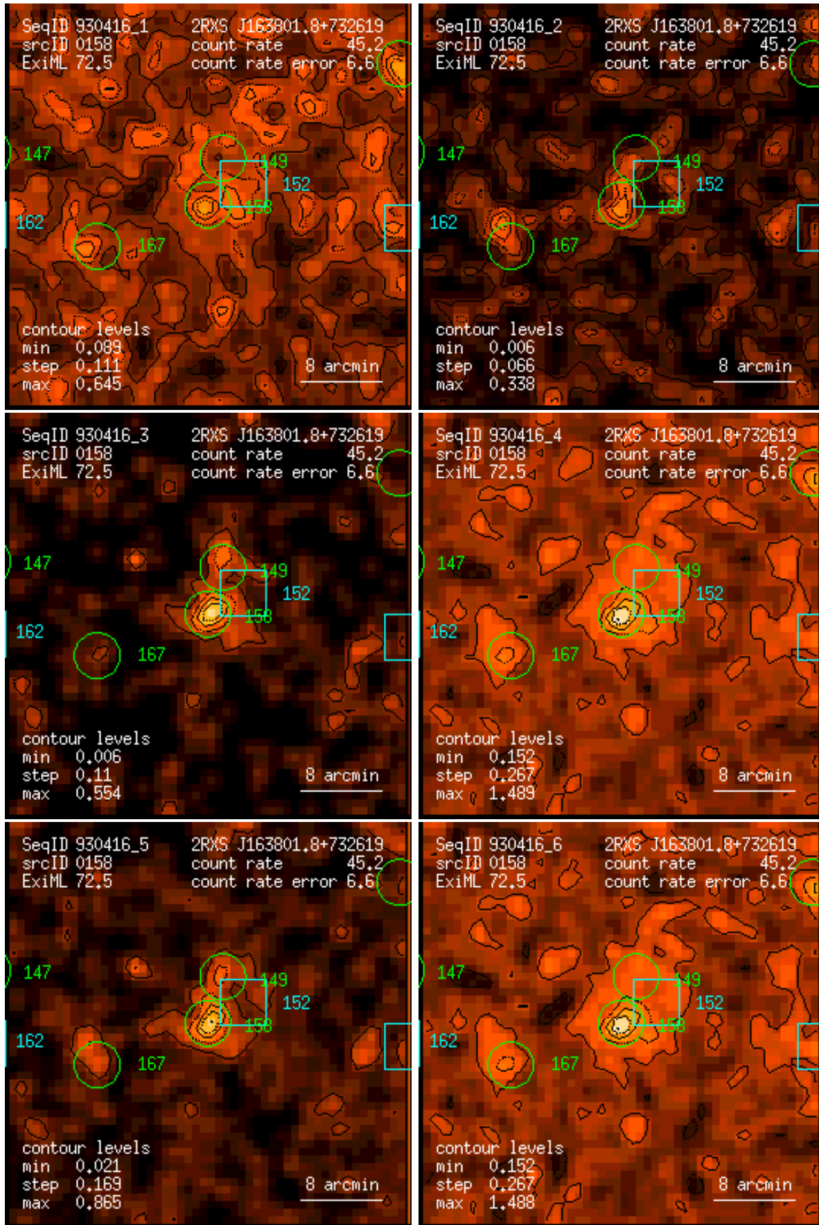
Figure 158: RASS 930416: detection 0158: band rate images, Gaussian filter: (1) PSPC channels 11 – 41, (2) 52 – 90, (3) 91 – 201, (4) 11 – 235, (5) 52 – 201, (6) 11 – 201. Broad band rates in counts/ks. Band rate contour levels in counts/ks/arcmin 2 .
