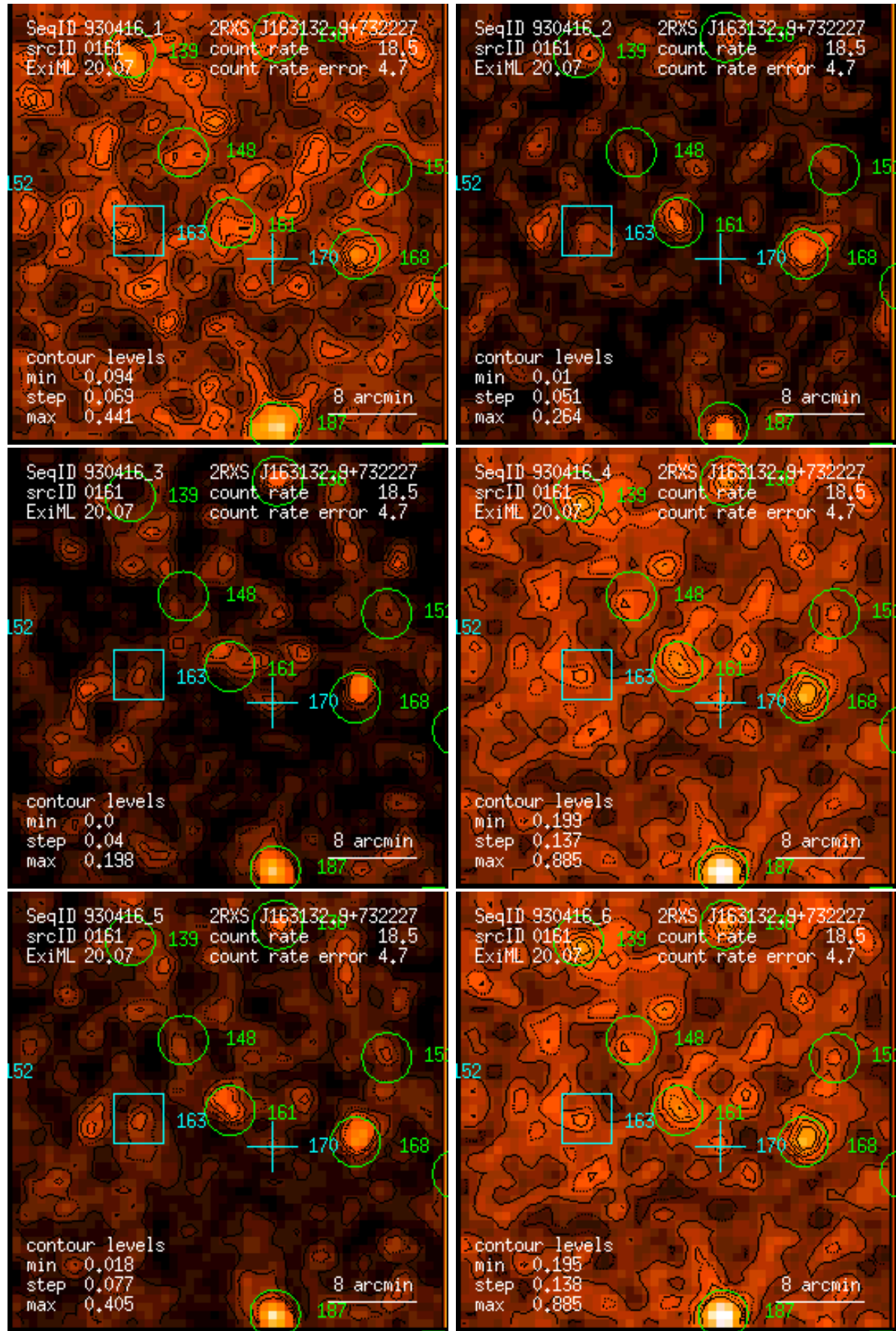
Figure 161: RASS 930416: detection 0161: band rate images, Gaussian filter: (1) PSPC channels 11 – 41, (2) 52 – 90, (3) 91 – 201, (4) 11 – 235, (5) 52 – 201, (6) 11 – 201. Broad band rates in counts/ks. Band rate contour levels in counts/ks/arcmin 2 .
