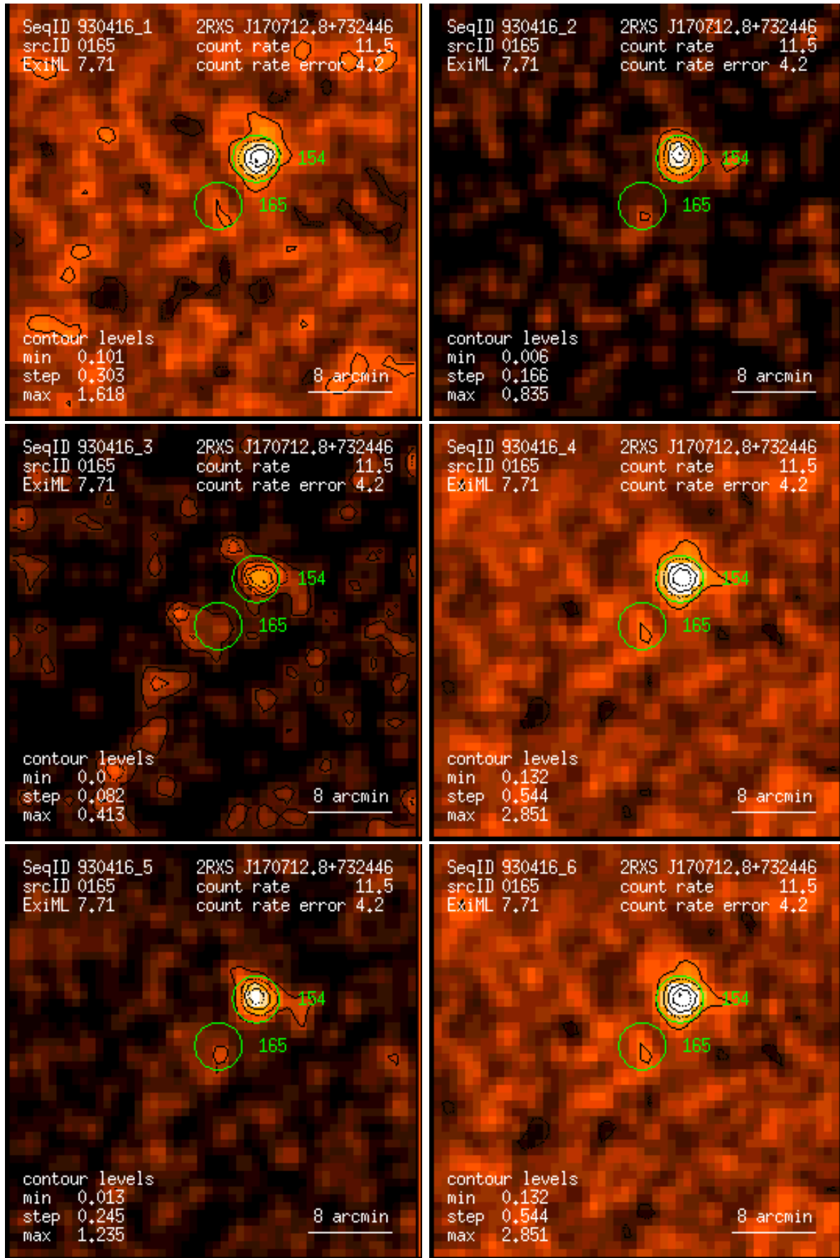
Figure 165: RASS 930416: detection 0165: band rate images, Gaussian filter: (1) PSPC channels 11 – 41, (2) 52 – 90, (3) 91 – 201, (4) 11 – 235, (5) 52 – 201, (6) 11 – 201. Broad band rates in counts/ks. Band rate contour levels in counts/ks/arcmin 2 .
