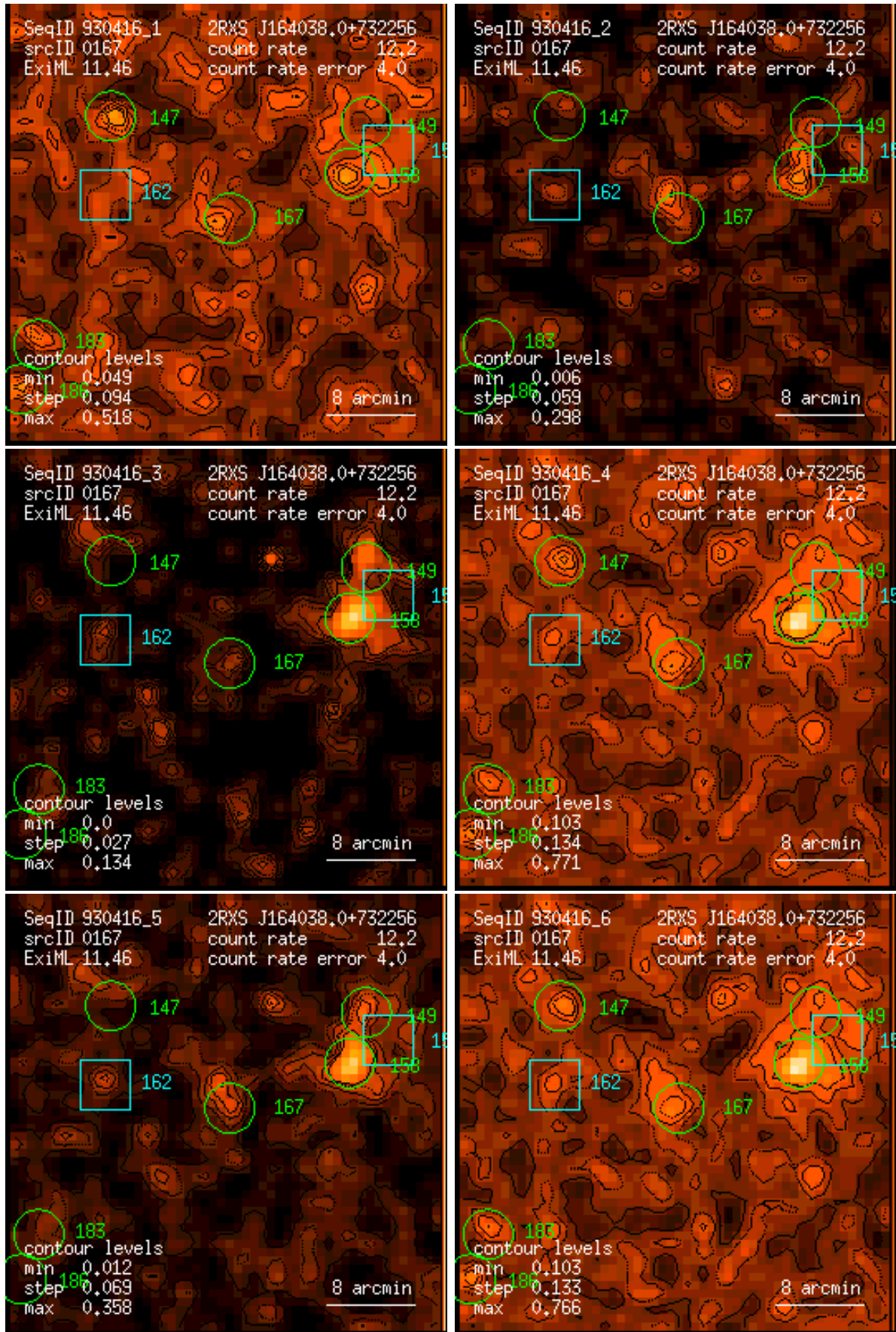
Figure 167: RASS 930416: detection 0167: band rate images, Gaussian filter: (1) PSPC channels 11 – 41, (2) 52 – 90, (3) 91 – 201, (4) 11 – 235, (5) 52 – 201, (6) 11 – 201. Broad band rates in counts/ks. Band rate contour levels in counts/ks/arcmin 2 .
