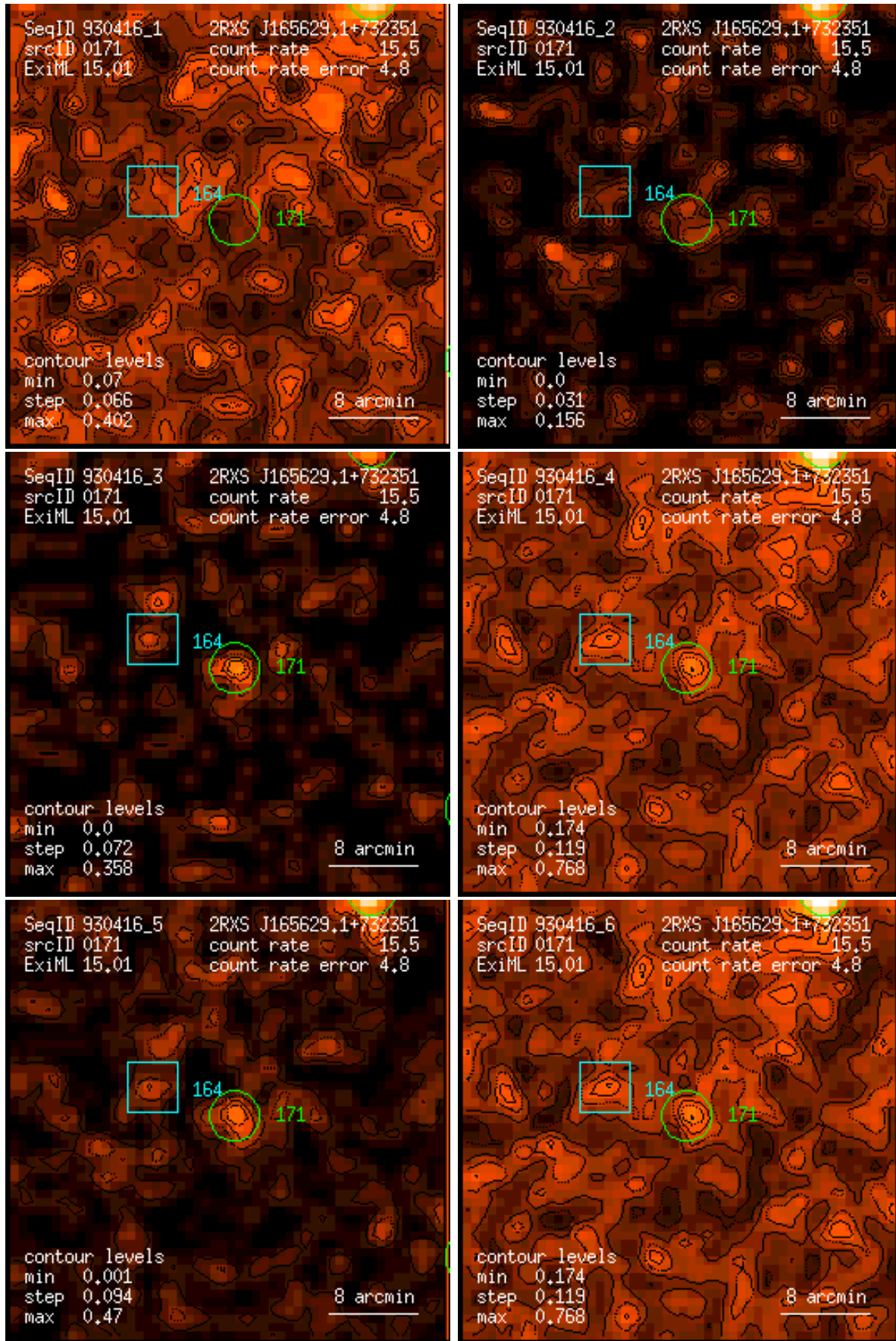
Figure 171: RASS 930416: detection 0171: band rate images, Gaussian filter: (1) PSPC channels 11 – 41, (2) 52 – 90, (3) 91 – 201, (4) 11 – 235, (5) 52 – 201, (6) 11 – 201. Broad band rates in counts/ks. Band rate contour levels in counts/ks/arcmin 2 .
