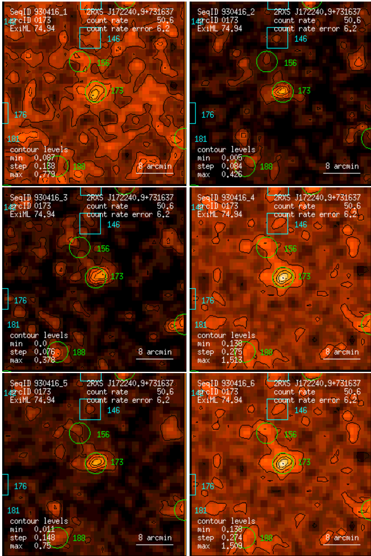
Figure 173: RASS 930416: detection 0173: band rate images, Gaussian filter: (1) PSPC channels 11 – 41, (2) 52 – 90, (3) 91 – 201, (4) 11 – 235, (5) 52 – 201, (6) 11 – 201. Broad band rates in counts/ks. Band rate contour levels in counts/ks/arcmin 2 .
