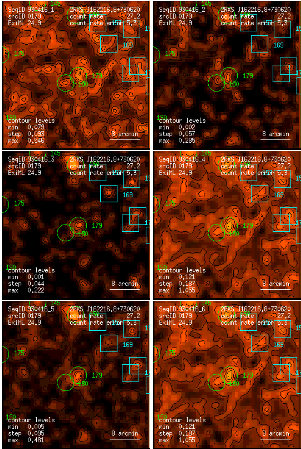
Figure 179: RASS 930416: detection 0179: band rate images, Gaussian filter: (1) PSPC channels 11 – 41, (2) 52 – 90, (3) 91 – 201, (4) 11 – 235, (5) 52 – 201, (6) 11 – 201. Broad band rates in counts/ks. Band rate contour levels in counts/ks/arcmin 2 .
