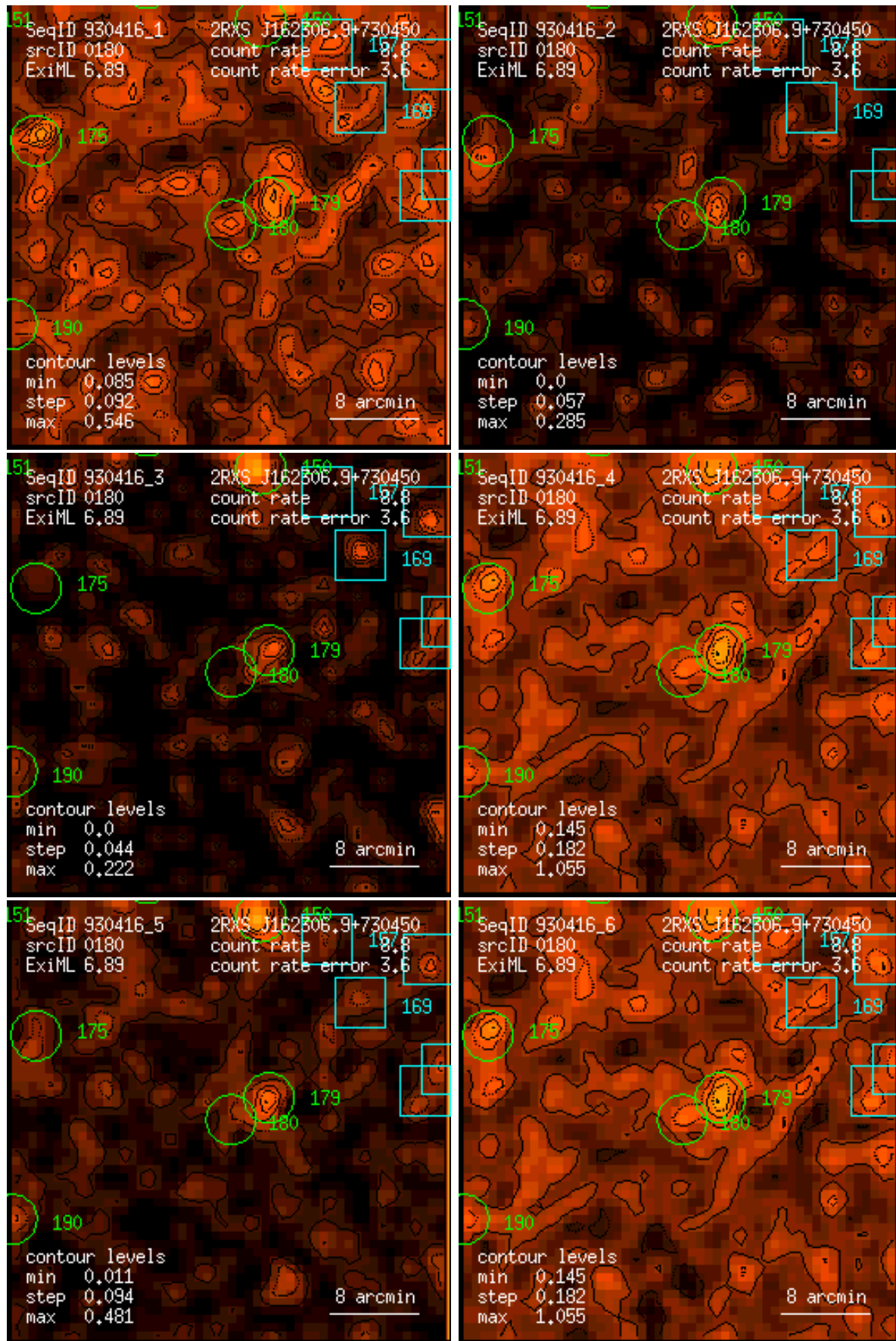
Figure 180: RASS 930416: detection 0180: band rate images, Gaussian filter: (1) PSPC channels 11 – 41, (2) 52 – 90, (3) 91 – 201, (4) 11 – 235, (5) 52 – 201, (6) 11 – 201. Broad band rates in counts/ks. Band rate contour levels in counts/ks/arcmin 2 .
