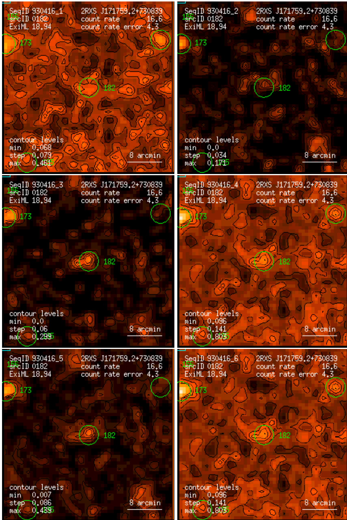
Figure 182: RASS 930416: detection 0182: band rate images, Gaussian filter: (1) PSPC channels 11 – 41, (2) 52 – 90, (3) 91 – 201, (4) 11 – 235, (5) 52 – 201, (6) 11 – 201. Broad band rates in counts/ks. Band rate contour levels in counts/ks/arcmin 2 .
