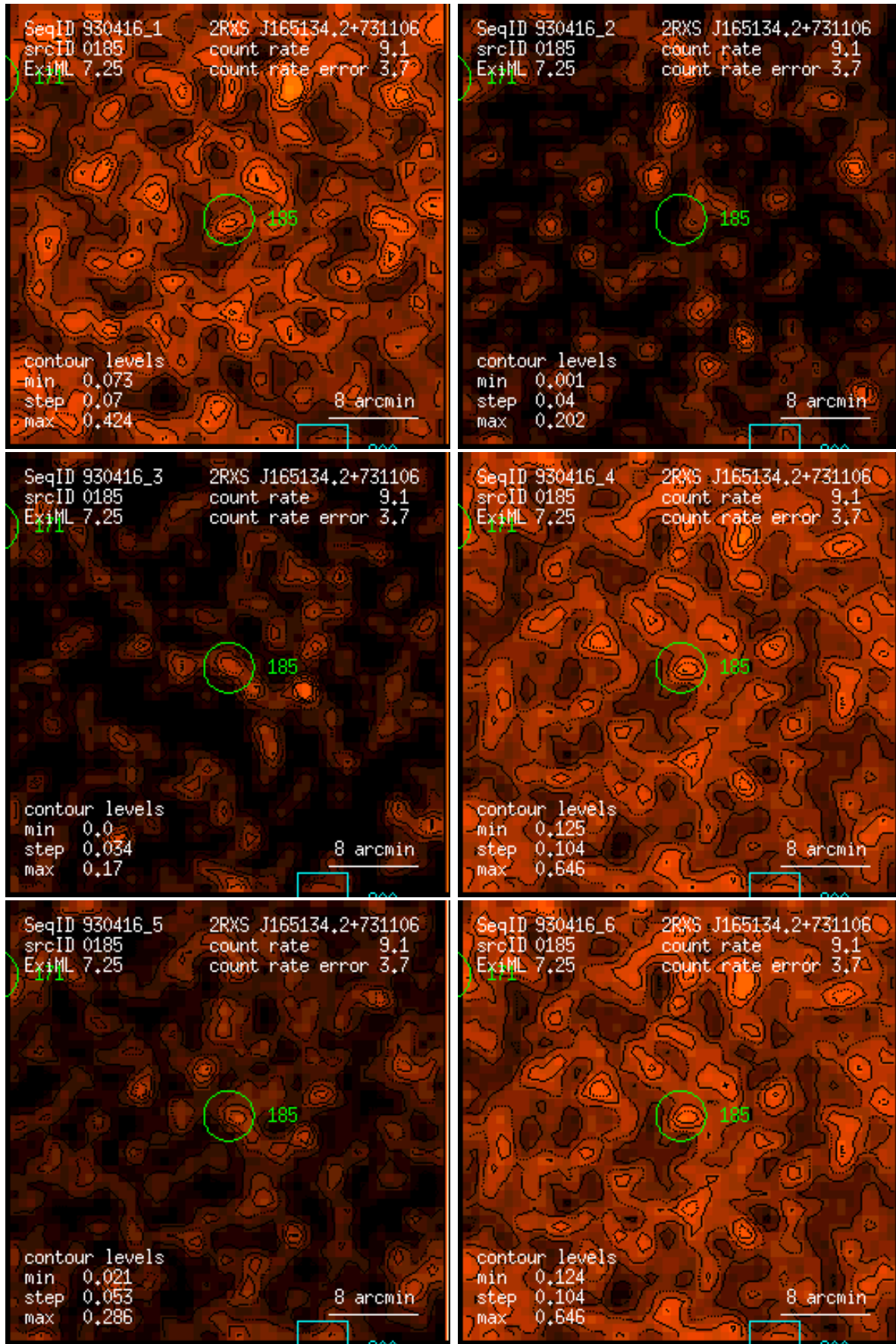
Figure 185: RASS 930416: detection 0185: band rate images, Gaussian filter: (1) PSPC channels 11 – 41, (2) 52 – 90, (3) 91 – 201, (4) 11 – 235, (5) 52 – 201, (6) 11 – 201. Broad band rates in counts/ks. Band rate contour levels in counts/ks/arcmin 2 .
