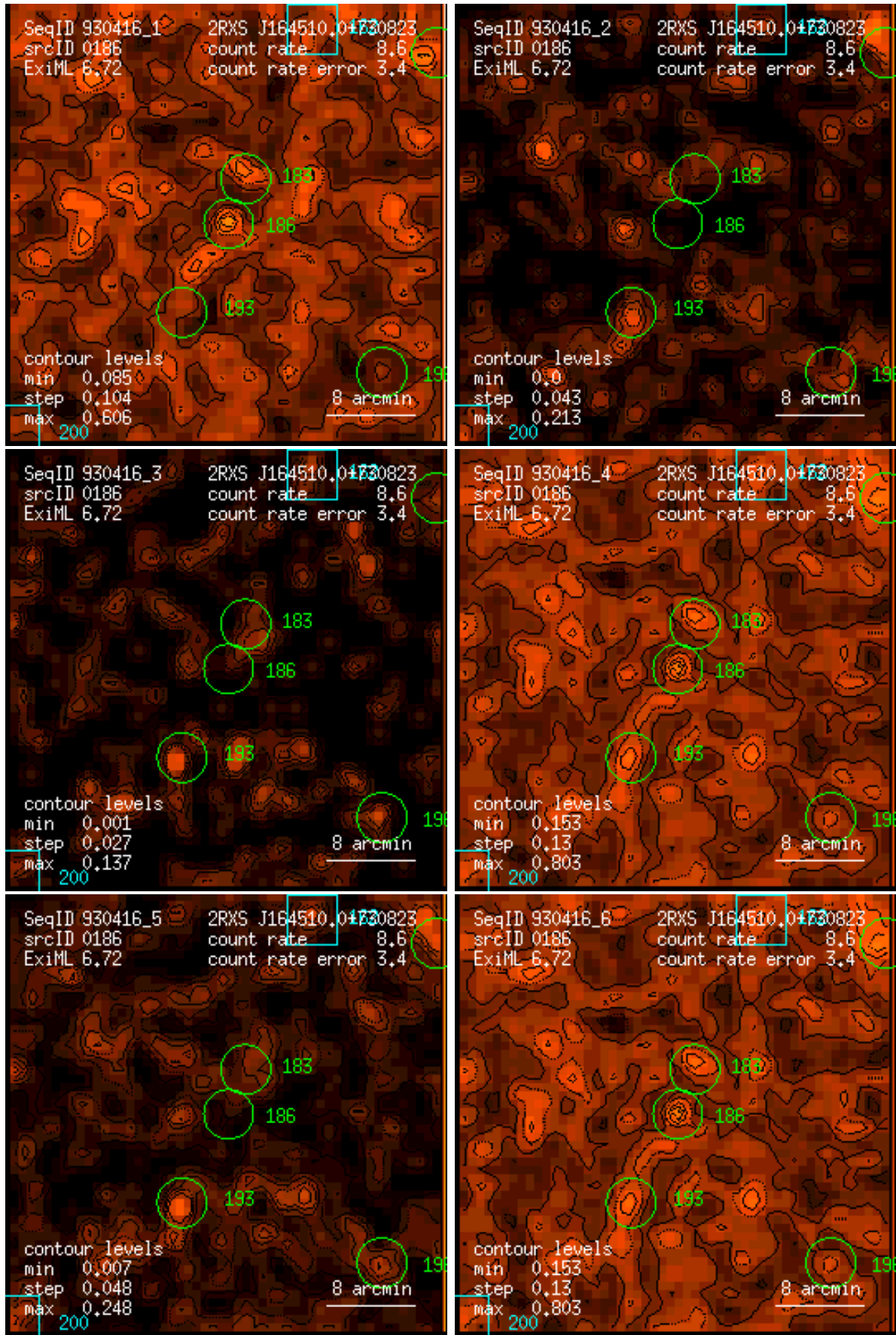
Figure 186: RASS 930416: detection 0186: band rate images, Gaussian filter: (1) PSPC channels 11 – 41, (2) 52 – 90, (3) 91 – 201, (4) 11 – 235, (5) 52 – 201, (6) 11 – 201. Broad band rates in counts/ks. Band rate contour levels in counts/ks/arcmin 2 .
