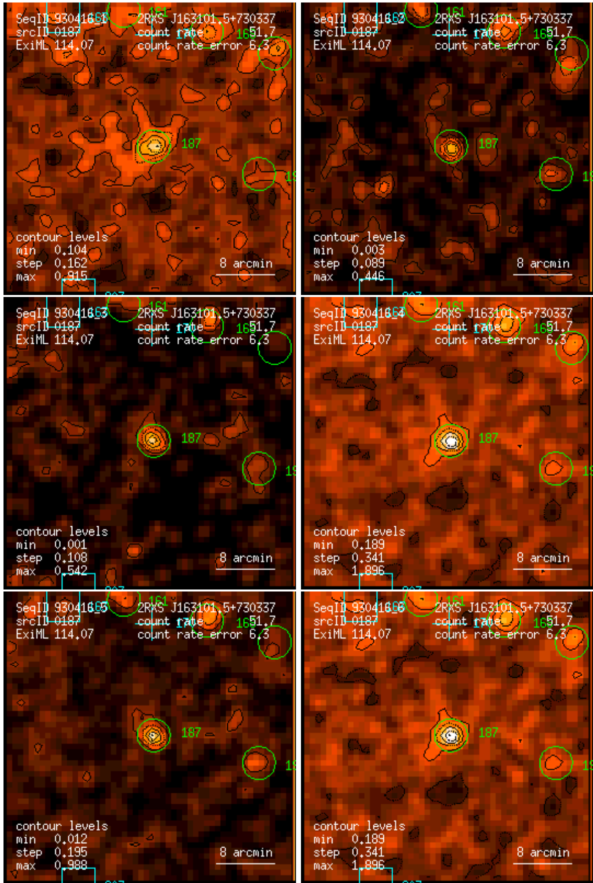
Figure 187: RASS 930416: detection 0187: band rate images, Gaussian filter: (1) PSPC channels 11 – 41, (2) 52 – 90, (3) 91 – 201, (4) 11 – 235, (5) 52 – 201, (6) 11 – 201. Broad band rates in counts/ks. Band rate contour levels in counts/ks/arcmin 2 .
