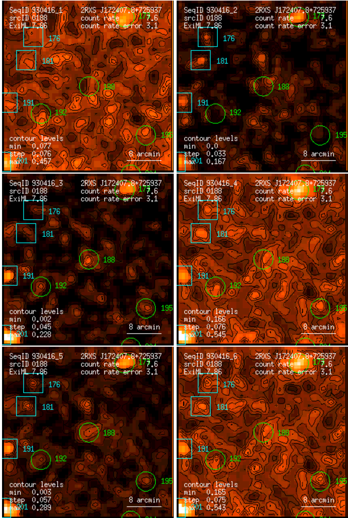
Figure 188: RASS 930416: detection 0188: band rate images, Gaussian filter: (1) PSPC channels 11 – 41, (2) 52 – 90, (3) 91 – 201, (4) 11 – 235, (5) 52 – 201, (6) 11 – 201. Broad band rates in counts/ks. Band rate contour levels in counts/ks/arcmin 2 .
