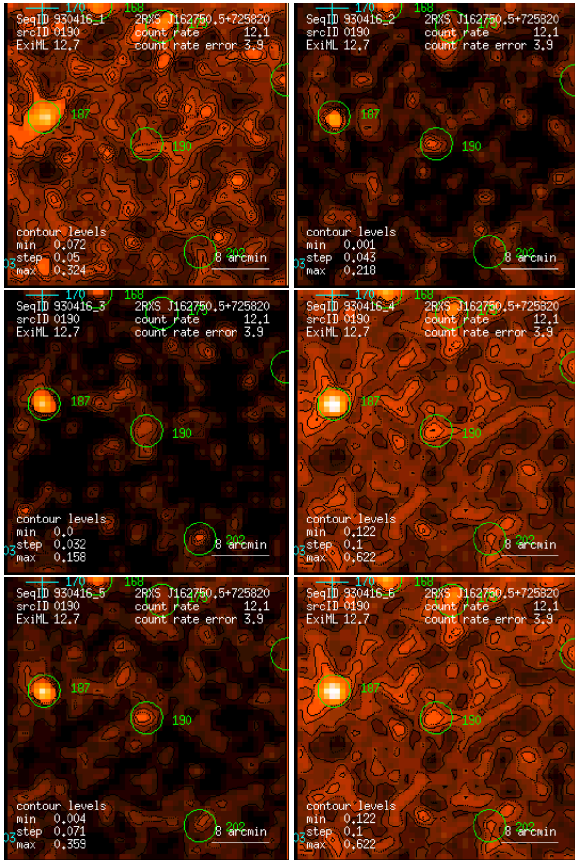
Figure 190: RASS 930416: detection 0190: band rate images, Gaussian filter: (1) PSPC channels 11 – 41, (2) 52 – 90, (3) 91 – 201, (4) 11 – 235, (5) 52 – 201, (6) 11 – 201. Broad band rates in counts/ks. Band rate contour levels in counts/ks/arcmin 2 .
