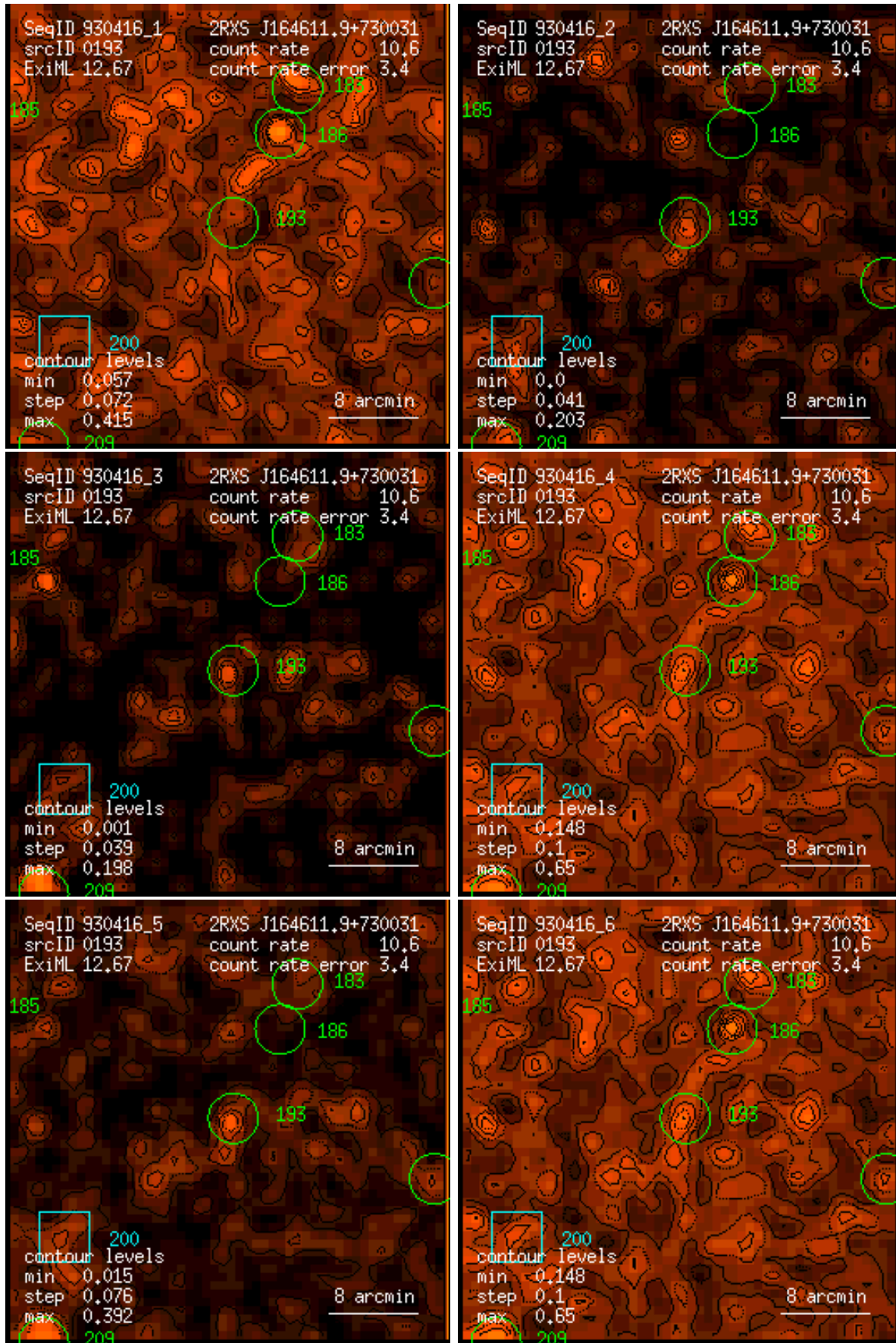
Figure 193: RASS 930416: detection 0193: band rate images, Gaussian filter: (1) PSPC channels 11 – 41, (2) 52 – 90, (3) 91 – 201, (4) 11 – 235, (5) 52 – 201, (6) 11 – 201. Broad band rates in counts/ks. Band rate contour levels in counts/ks/arcmin 2 .
