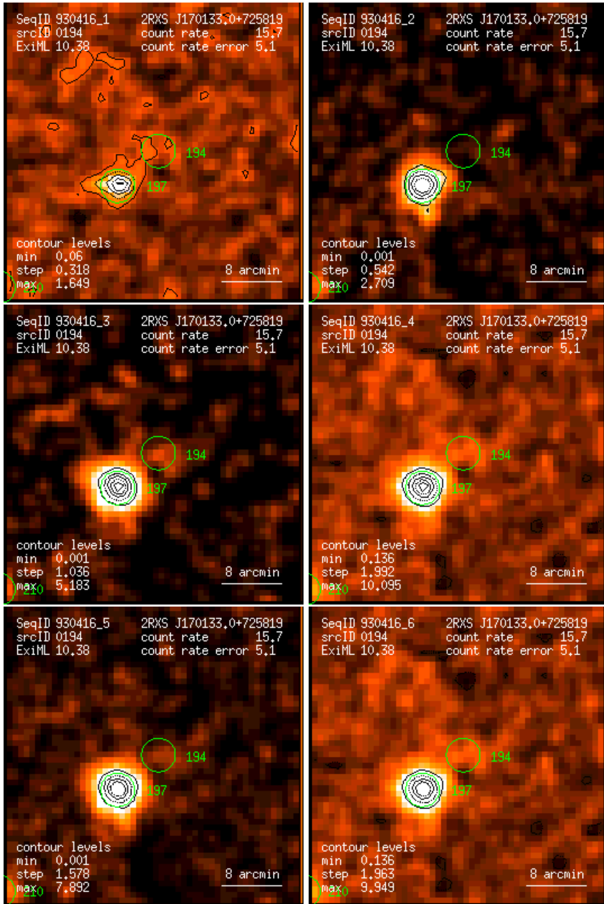
Figure 194: RASS 930416: detection 0194: band rate images, Gaussian filter: (1) PSPC channels 11 – 41, (2) 52 – 90, (3) 91 – 201, (4) 11 – 235, (5) 52 – 201, (6) 11 – 201. Broad band rates in counts/ks. Band rate contour levels in counts/ks/arcmin 2 .
