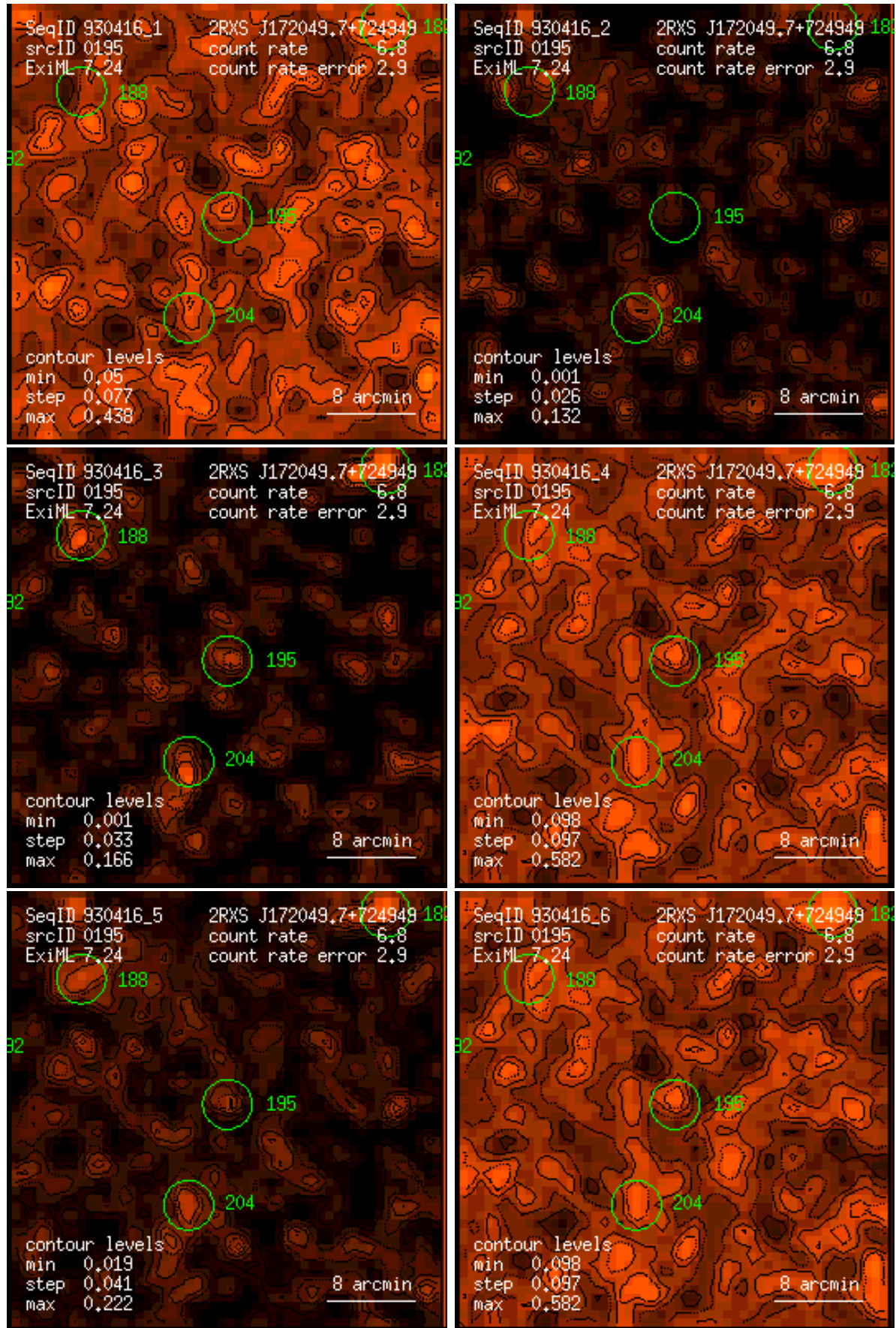
Figure 195: RASS 930416: detection 0195: band rate images, Gaussian filter: (1) PSPC channels 11 – 41, (2) 52 – 90, (3) 91 – 201, (4) 11 – 235, (5) 52 – 201, (6) 11 – 201. Broad band rates in counts/ks. Band rate contour levels in counts/ks/arcmin 2 .
