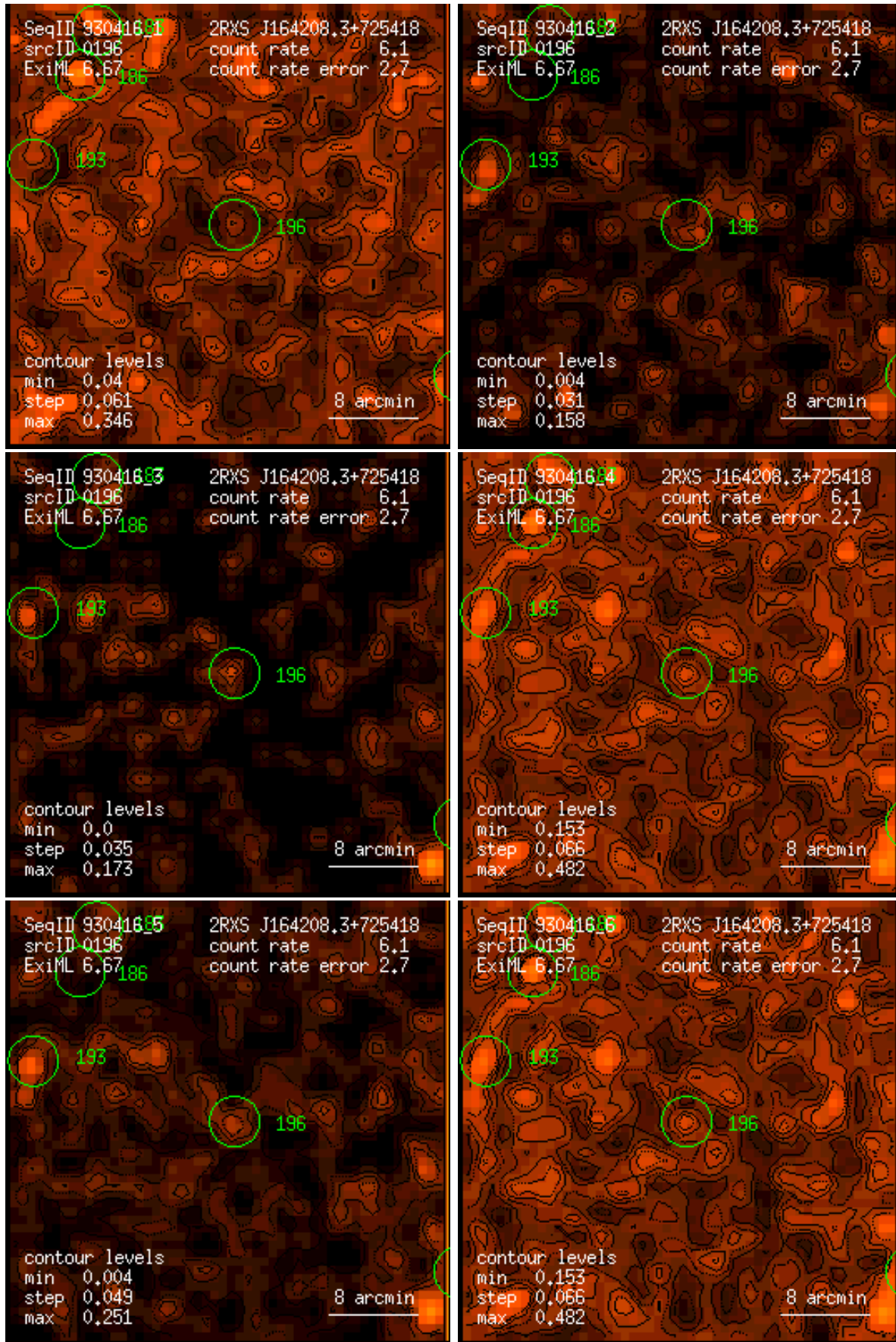
Figure 196: RASS 930416: detection 0196: band rate images, Gaussian filter: (1) PSPC channels 11 – 41, (2) 52 – 90, (3) 91 – 201, (4) 11 – 235, (5) 52 – 201, (6) 11 – 201. Broad band rates in counts/ks. Band rate contour levels in counts/ks/arcmin 2 .
