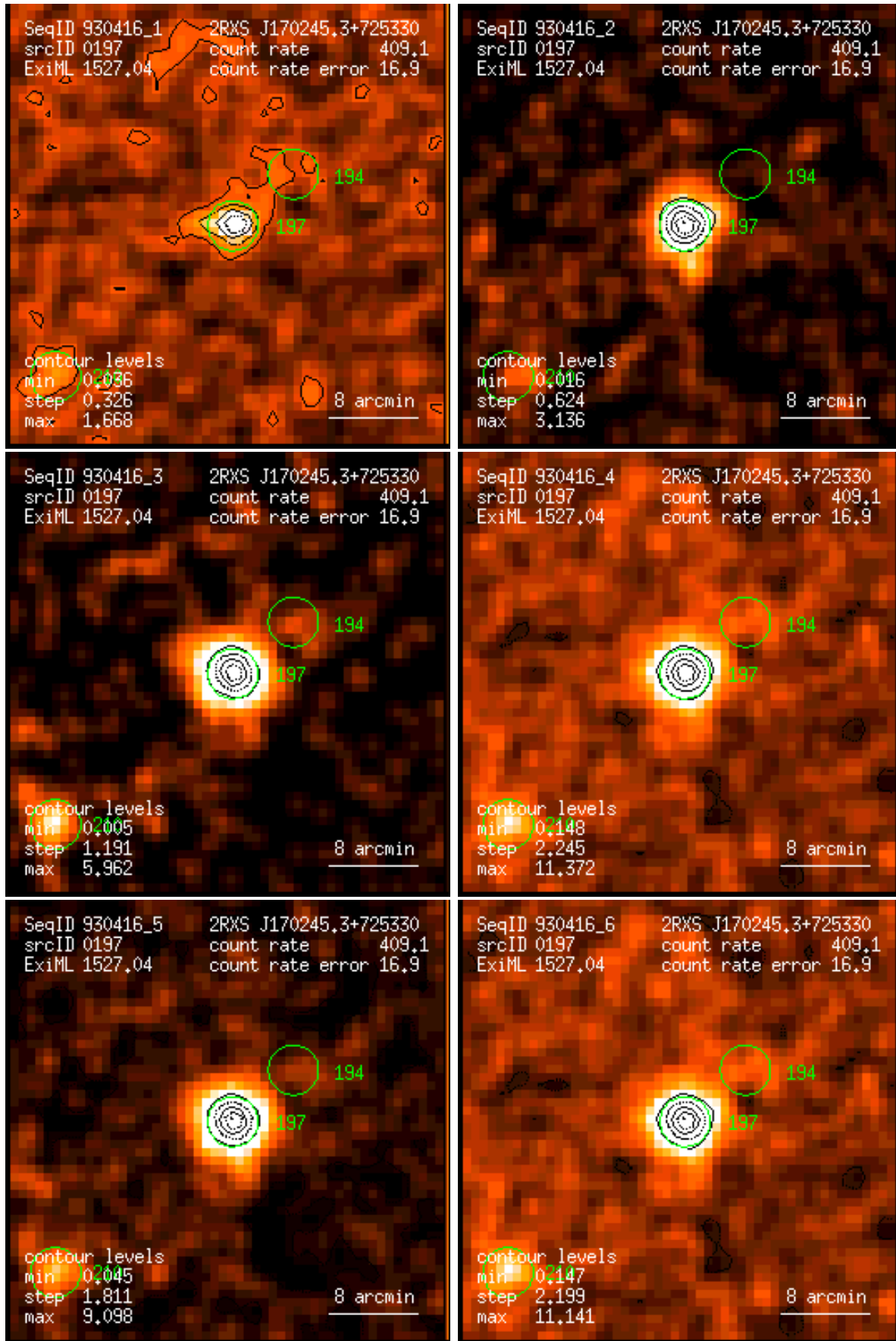
Figure 197: RASS 930416: detection 0197: band rate images, Gaussian filter: (1) PSPC channels 11 – 41, (2) 52 – 90, (3) 91 – 201, (4) 11 – 235, (5) 52 – 201, (6) 11 – 201. Broad band rates in counts/ks. Band rate contour levels in counts/ks/arcmin 2 .
