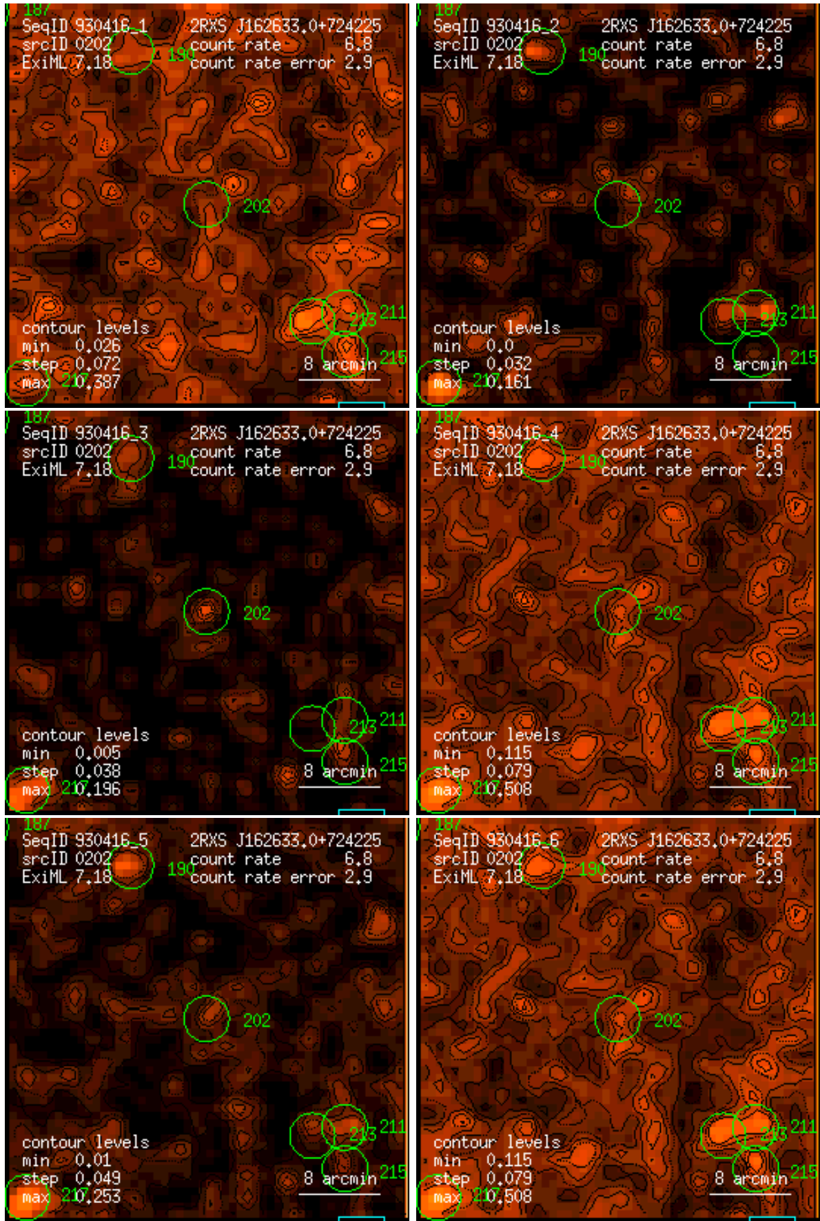
Figure 202: RASS 930416: detection 0202: band rate images, Gaussian filter: (1) PSPC channels 11 – 41, (2) 52 – 90, (3) 91 – 201, (4) 11 – 235, (5) 52 – 201, (6) 11 – 201. Broad band rates in counts/ks. Band rate contour levels in counts/ks/arcmin 2 .
