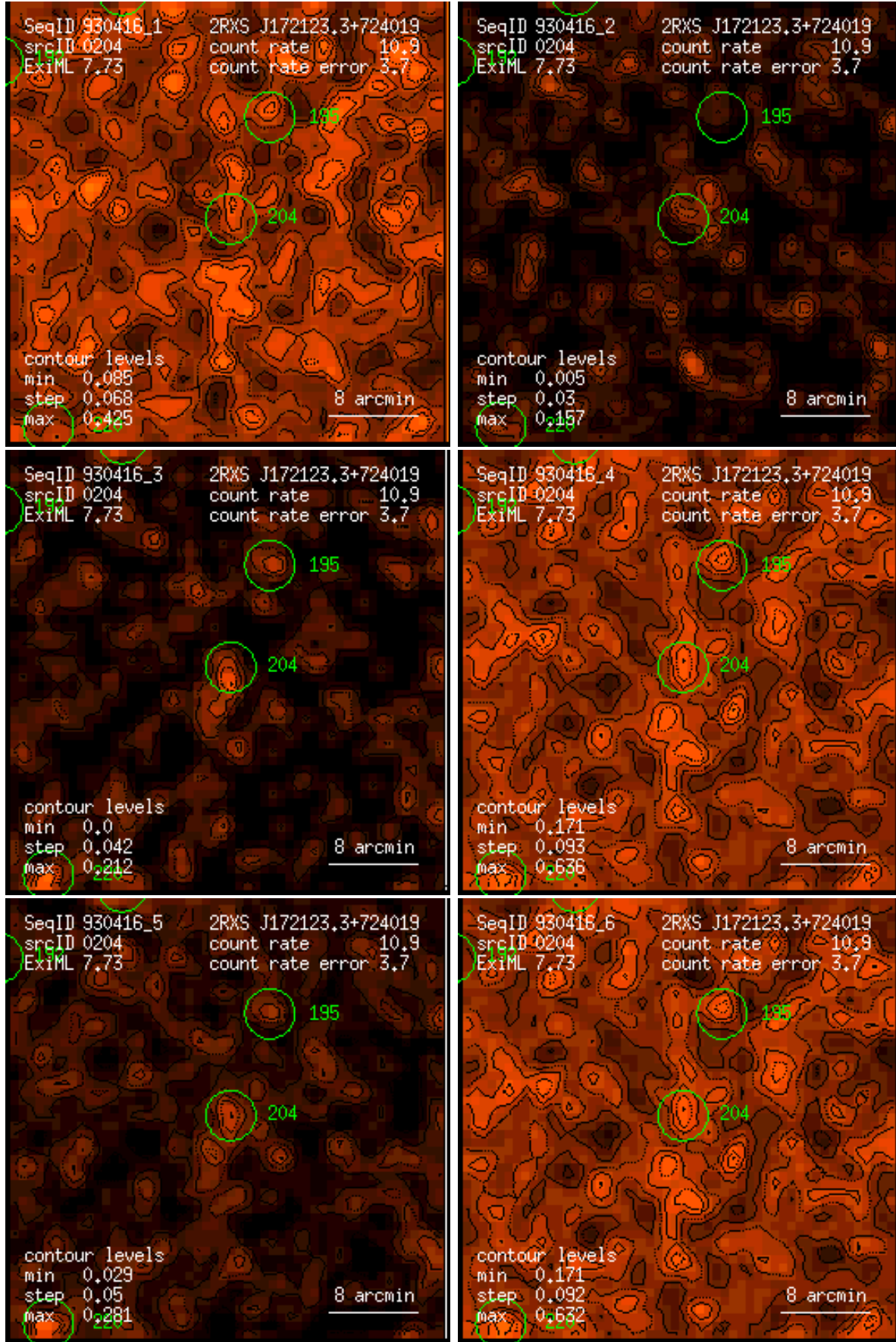
Figure 204: RASS 930416: detection 0204: band rate images, Gaussian filter: (1) PSPC channels 11 – 41, (2) 52 – 90, (3) 91 – 201, (4) 11 – 235, (5) 52 – 201, (6) 11 – 201. Broad band rates in counts/ks. Band rate contour levels in counts/ks/arcmin 2 .
