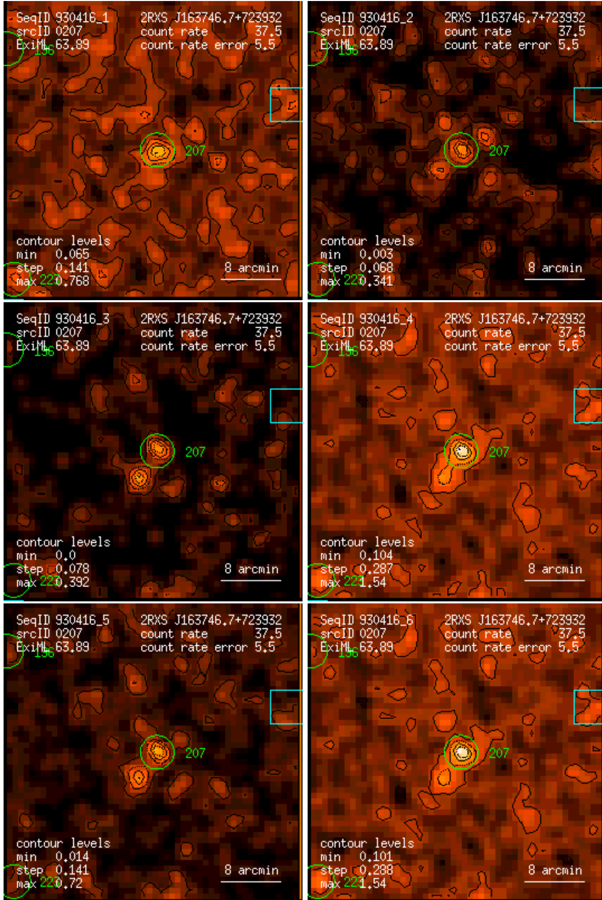
Figure 207: RASS 930416: detection 0207: band rate images, Gaussian filter: (1) PSPC channels 11 – 41, (2) 52 – 90, (3) 91 – 201, (4) 11 – 235, (5) 52 – 201, (6) 11 – 201. Broad band rates in counts/ks. Band rate contour levels in counts/ks/arcmin 2 .
