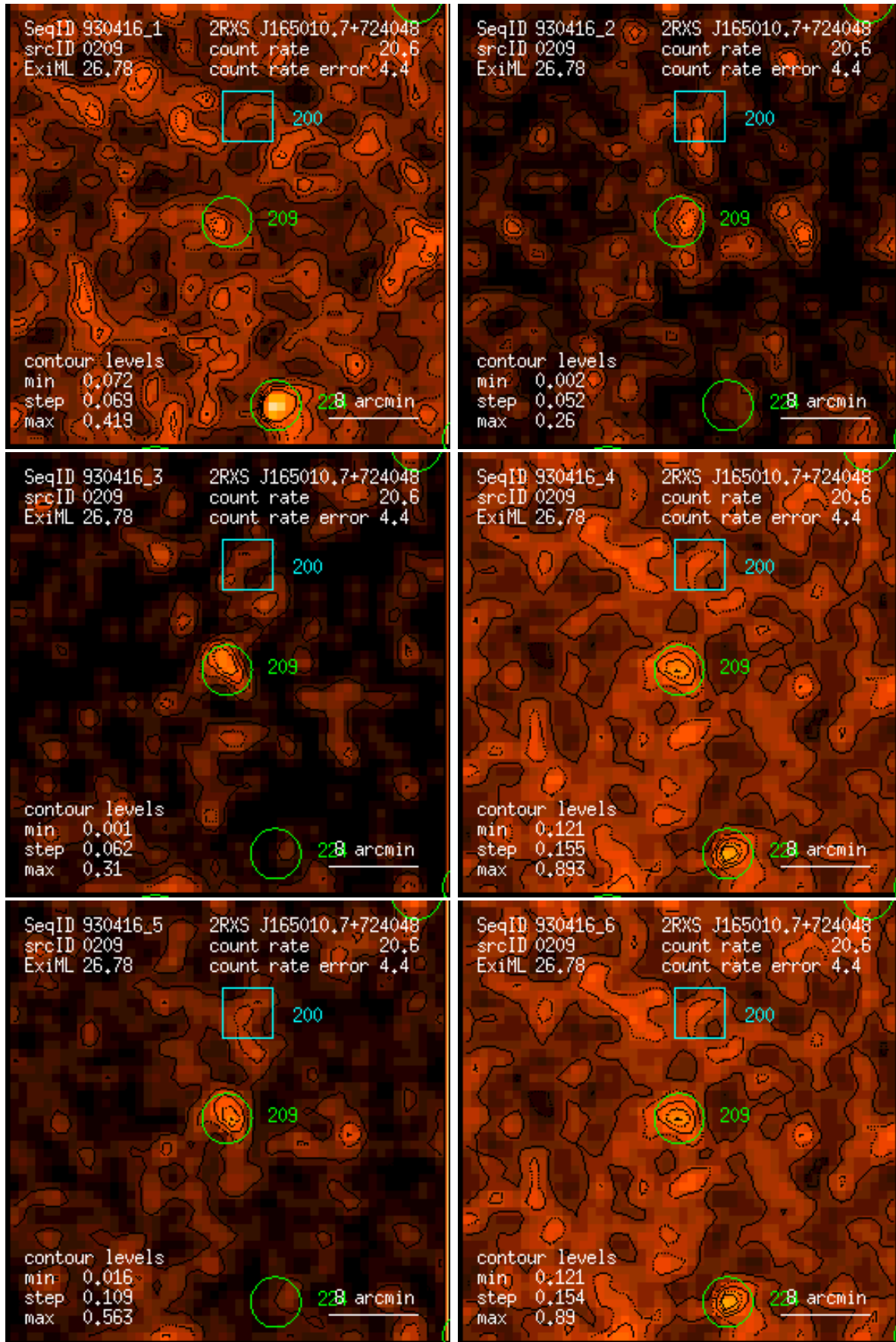
Figure 209: RASS 930416: detection 0209: band rate images, Gaussian filter: (1) PSPC channels 11 – 41, (2) 52 – 90, (3) 91 – 201, (4) 11 – 235, (5) 52 – 201, (6) 11 – 201. Broad band rates in counts/ks. Band rate contour levels in counts/ks/arcmin 2 .
