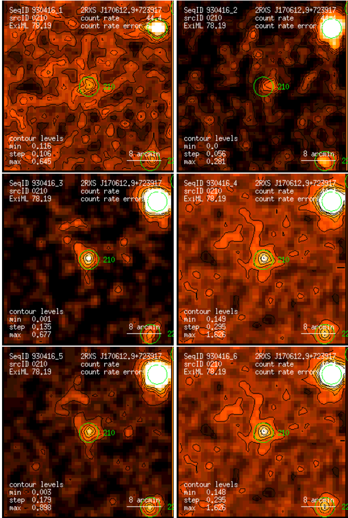
Figure 210: RASS 930416: detection 0210: band rate images, Gaussian filter: (1) PSPC channels 11 – 41, (2) 52 – 90, (3) 91 – 201, (4) 11 – 235, (5) 52 – 201, (6) 11 – 201. Broad band rates in counts/ks. Band rate contour levels in counts/ks/arcmin 2 .
