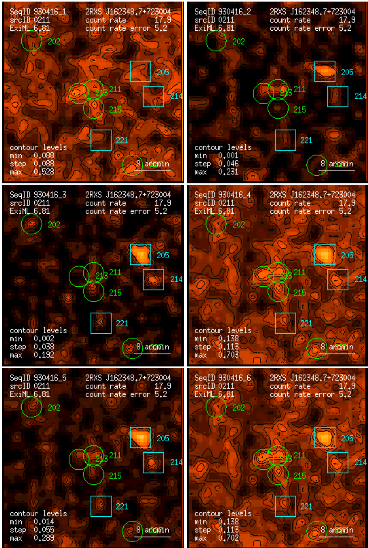
Figure 211: RASS 930416: detection 0211: band rate images, Gaussian filter: (1) PSPC channels 11 – 41, (2) 52 – 90, (3) 91 – 201, (4) 11 – 235, (5) 52 – 201, (6) 11 – 201. Broad band rates in counts/ks. Band rate contour levels in counts/ks/arcmin 2 .
