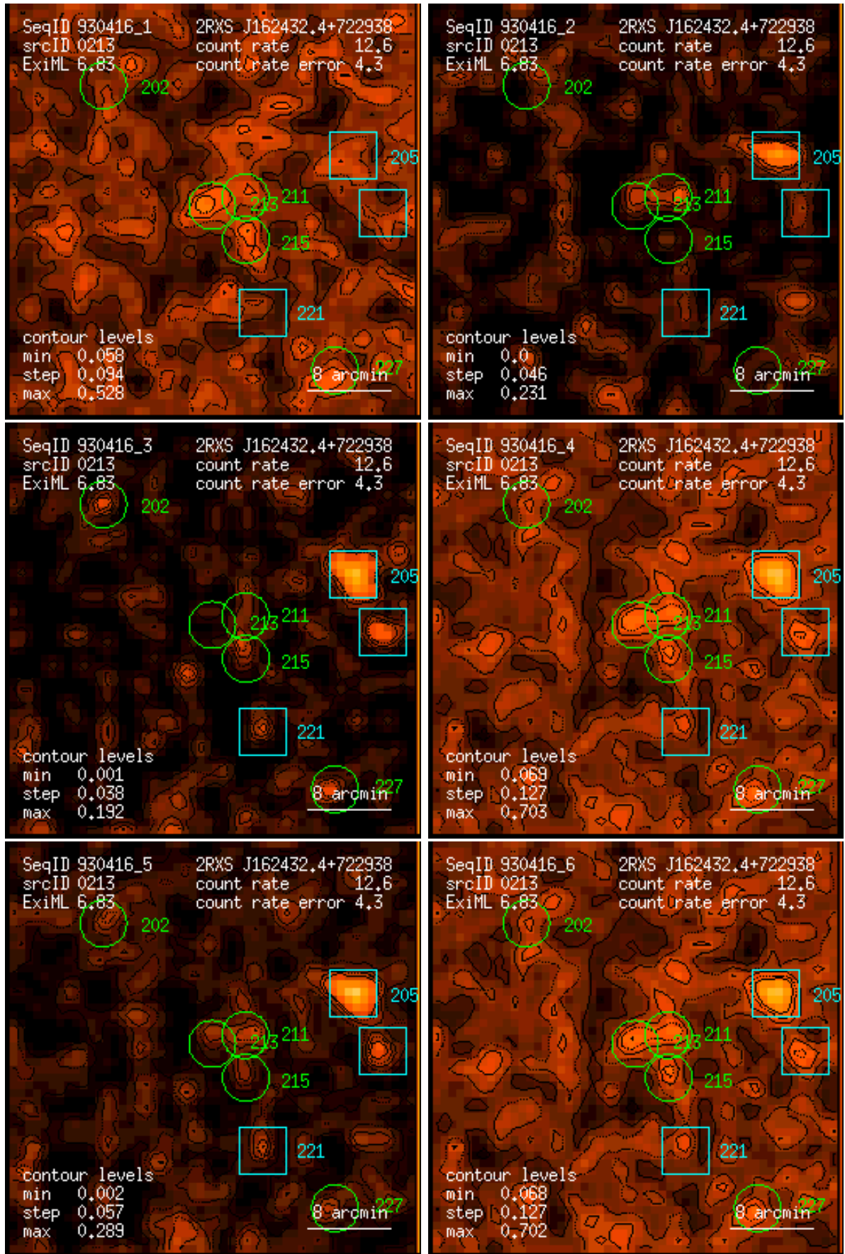
Figure 213: RASS 930416: detection 0213: band rate images, Gaussian filter: (1) PSPC channels 11 – 41, (2) 52 – 90, (3) 91 – 201, (4) 11 – 235, (5) 52 – 201, (6) 11 – 201. Broad band rates in counts/ks. Band rate contour levels in counts/ks/arcmin 2 .
